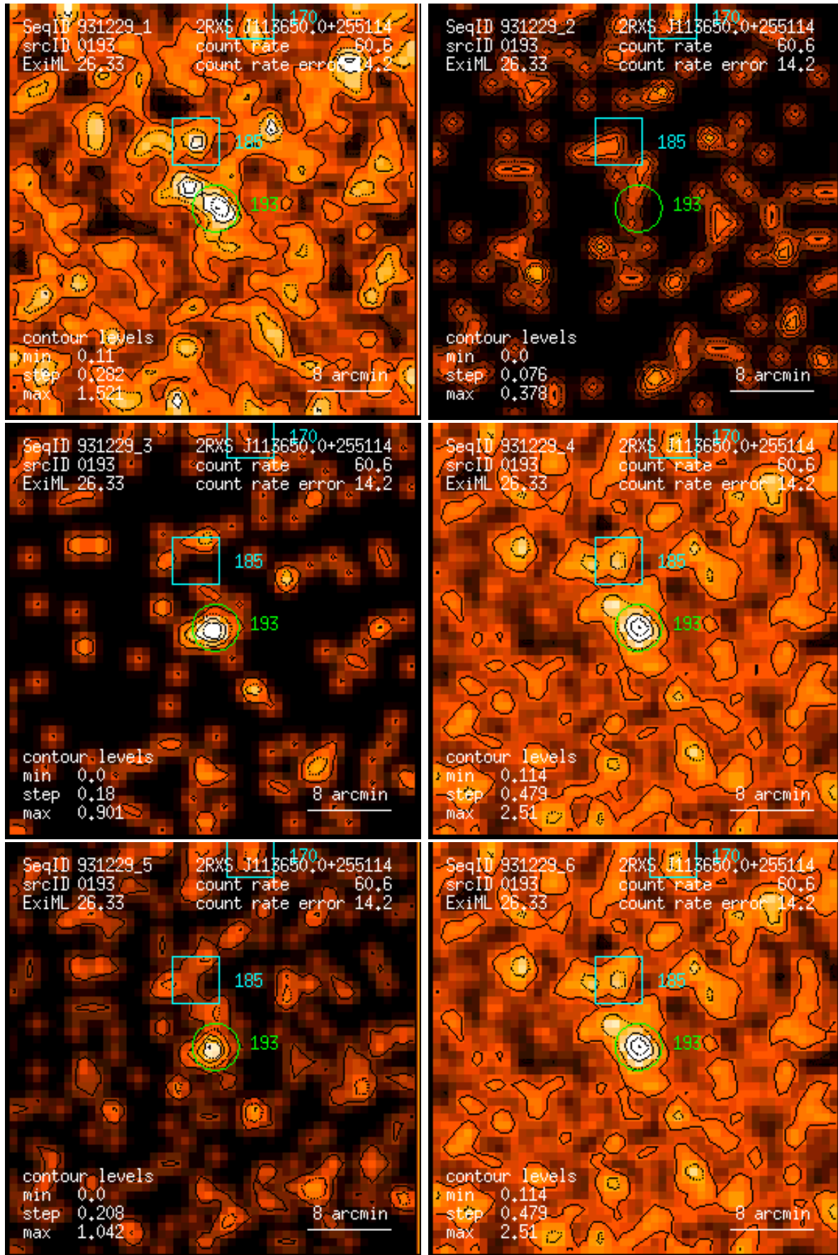
Figure 193: RASS 931229: detection 0193: band rate images, Gaussian filter: (1) PSPC channels 11 – 41, (2) 52 – 90, (3) 91 – 201, (4) 11 – 235, (5) 52 – 201, (6) 11 – 201. Broad band rates in counts/ks. Band rate contour levels in counts/ks/arcmin 2 .
