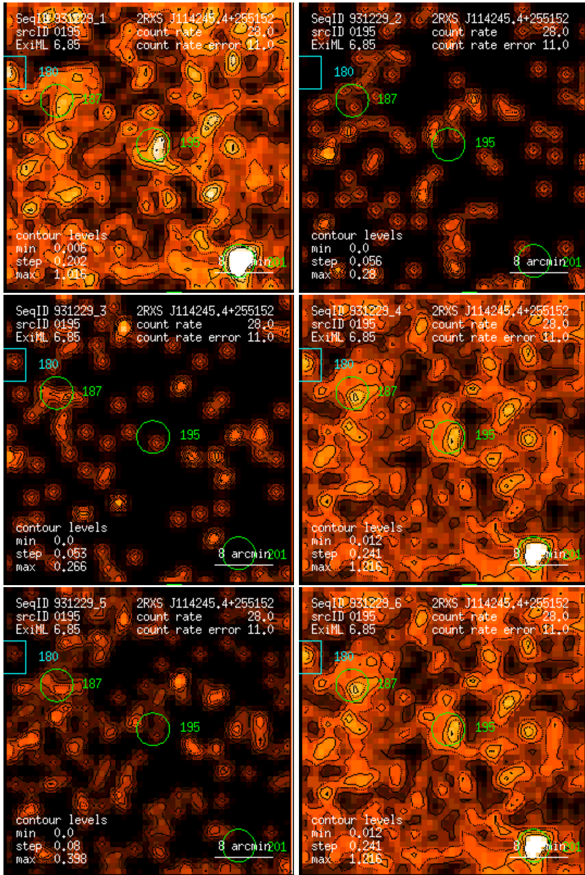
Figure 195: RASS 931229: detection 0195: band rate images, Gaussian filter: (1) PSPC channels 11 – 41, (2) 52 – 90, (3) 91 – 201, (4) 11 – 235, (5) 52 – 201, (6) 11 – 201. Broad band rates in counts/ks. Band rate contour levels in counts/ks/arcmin 2 .
