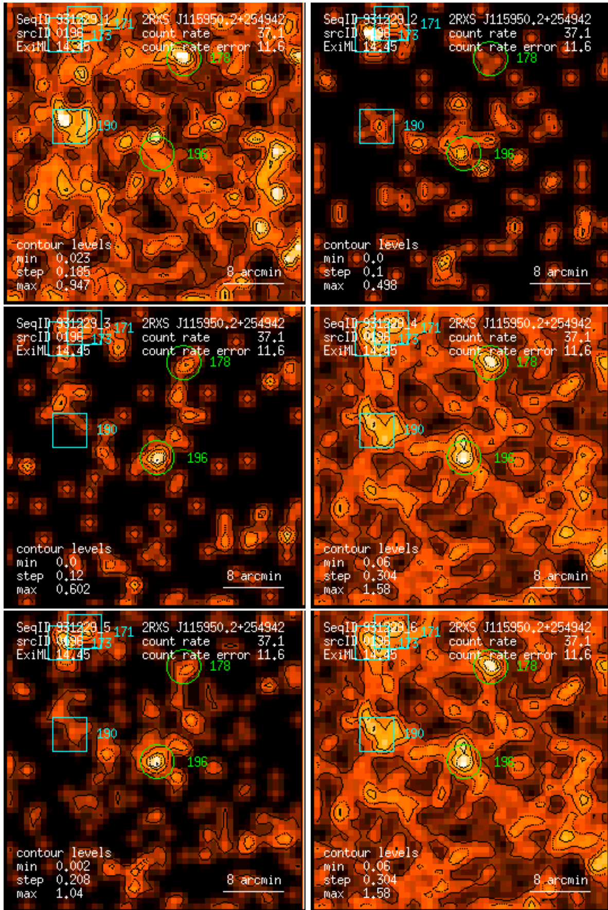
Figure 196: RASS 931229: detection 0196: band rate images, Gaussian filter: (1) PSPC channels 11 – 41, (2) 52 – 90, (3) 91 – 201, (4) 11 – 235, (5) 52 – 201, (6) 11 – 201. Broad band rates in counts/ks. Band rate contour levels in counts/ks/arcmin 2 .
