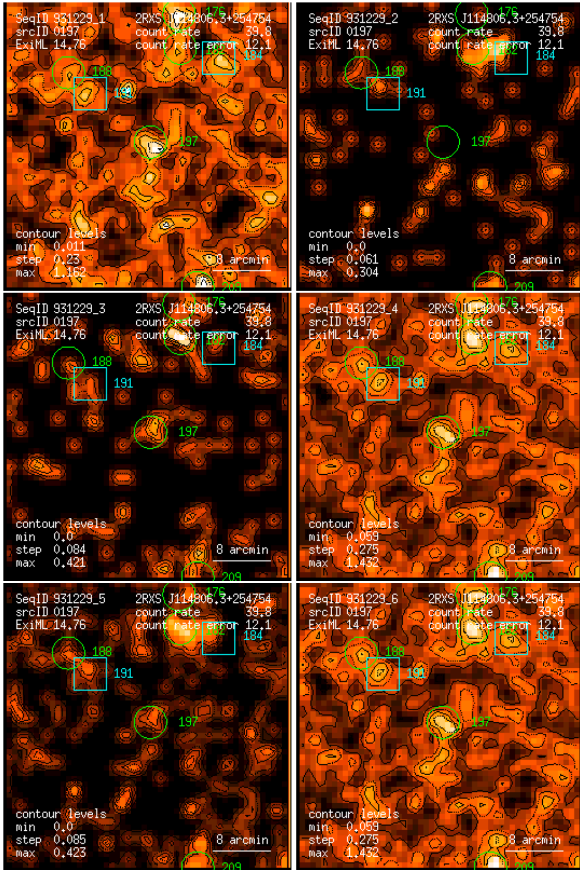
Figure 197: RASS 931229: detection 0197: band rate images, Gaussian filter: (1) PSPPC channels 11 – 41, (2) 52 – 90, (3) 91 – 201, (4) 11 – 235, (5) 52 – 201, (6) 11 – 201. Broad band rates in counts/ks. Band rate contour levels in counts/ks/arcmin 2 .
