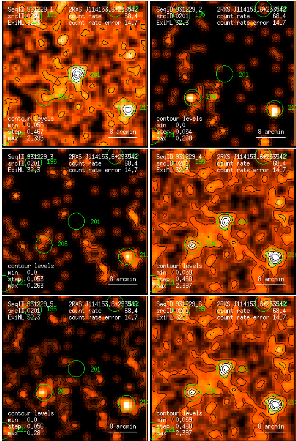
Figure 201: RASS 931229: detection 0201: band rate images, Gaussian filter: (1) PSPC channels 11 – 41, (2) 52 – 90, (3) 91 – 201, (4) 11 – 235, (5) 52 – 201, (6) 11 – 201. Broad band rates in counts/ks. Band rate contour levels in counts/ks/arcmin 2 .
