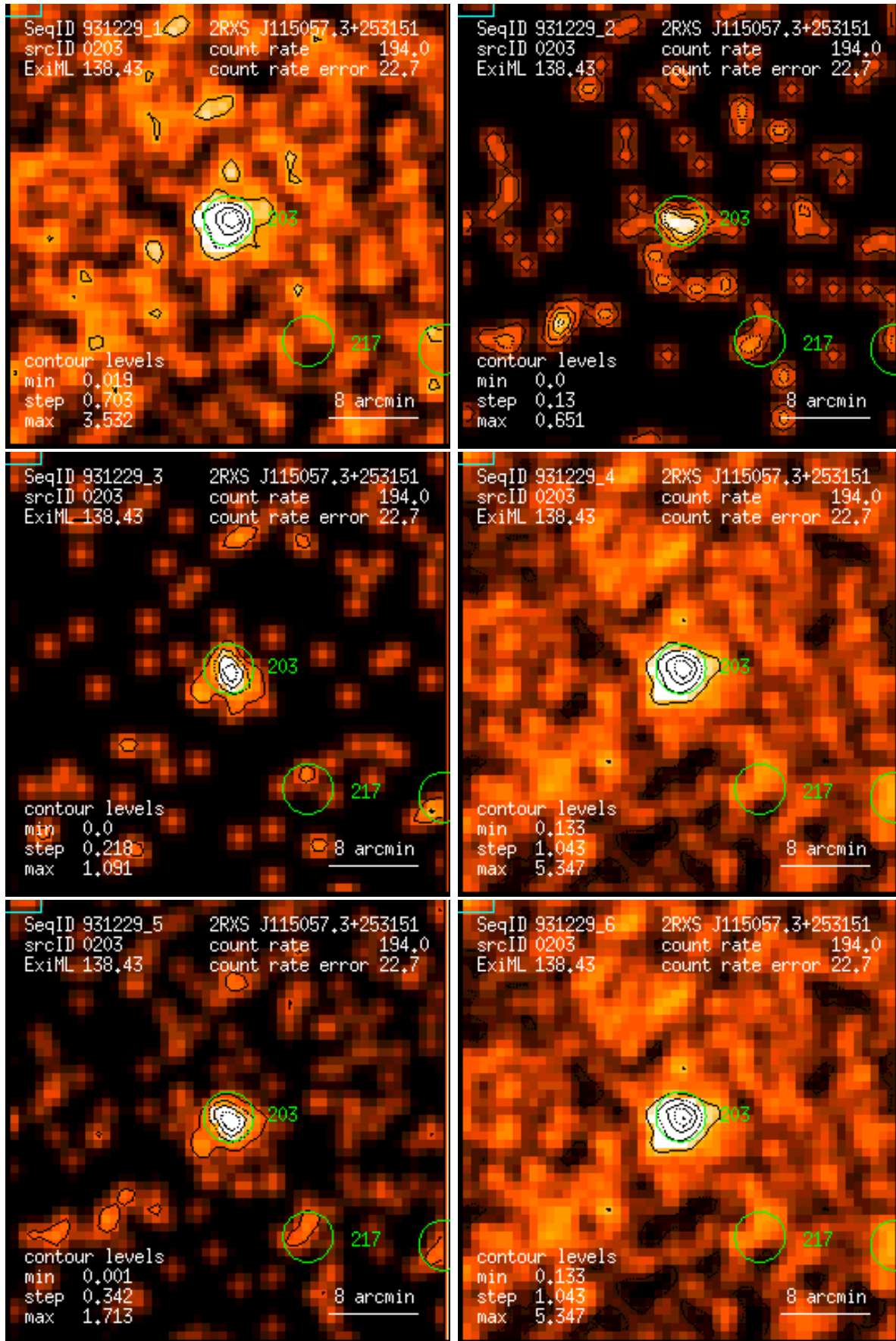
Figure 203: RASS 931229: detection 0203: band rate images, Gaussian filter: (1) PSPC channels 11 – 41, (2) 52 – 90, (3) 91 – 201, (4) 11 – 235, (5) 52 – 201, (6) 11 – 201. Broad band rates in counts/ks. Band rate contour levels in counts/ks/arcmin 2 .
