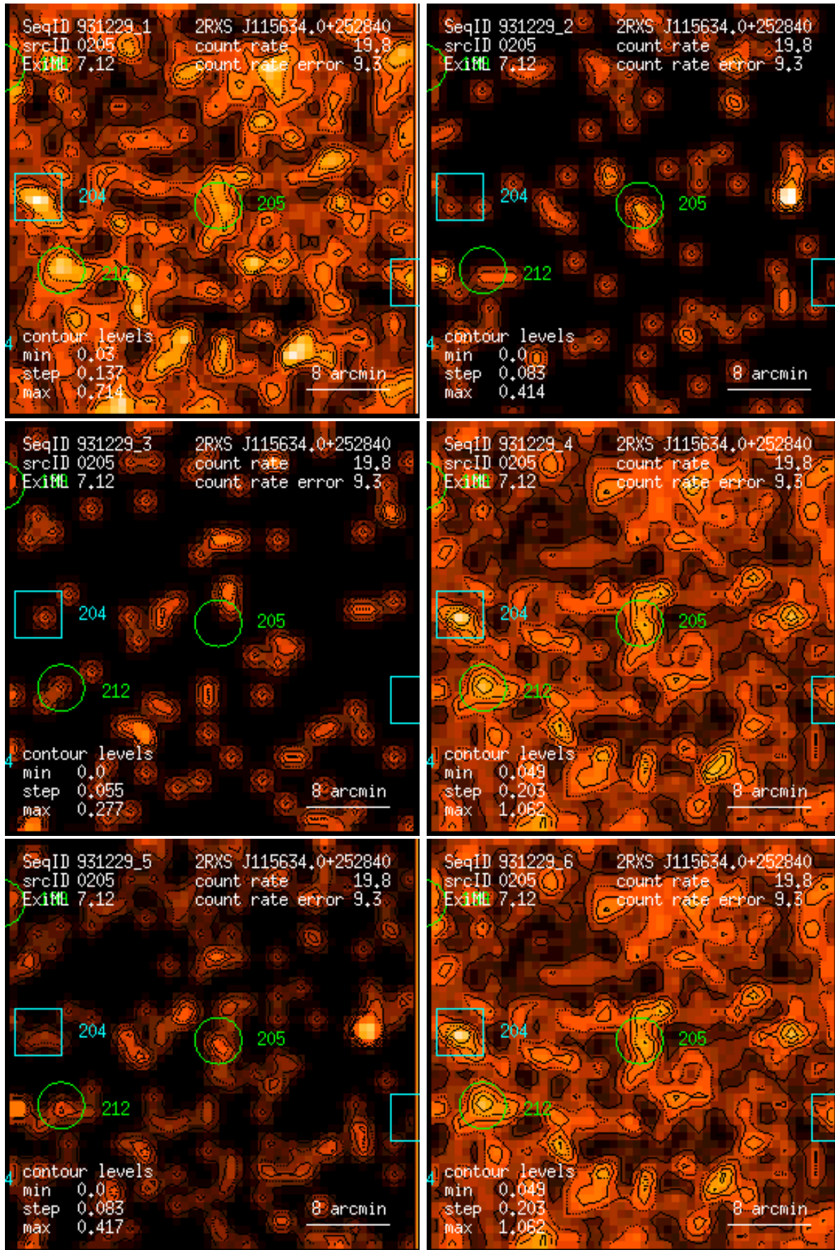
Figure 205: RASS 931229: detection 0205: band rate images, Gaussian filter: (1) PSPC channels 11 – 41, (2) 52 – 90, (3) 91 – 201, (4) 11 – 235, (5) 52 – 201, (6) 11 – 201. Broad band rates in counts/ks. Band rate contour levels in counts/ks/arcmin 2 .
