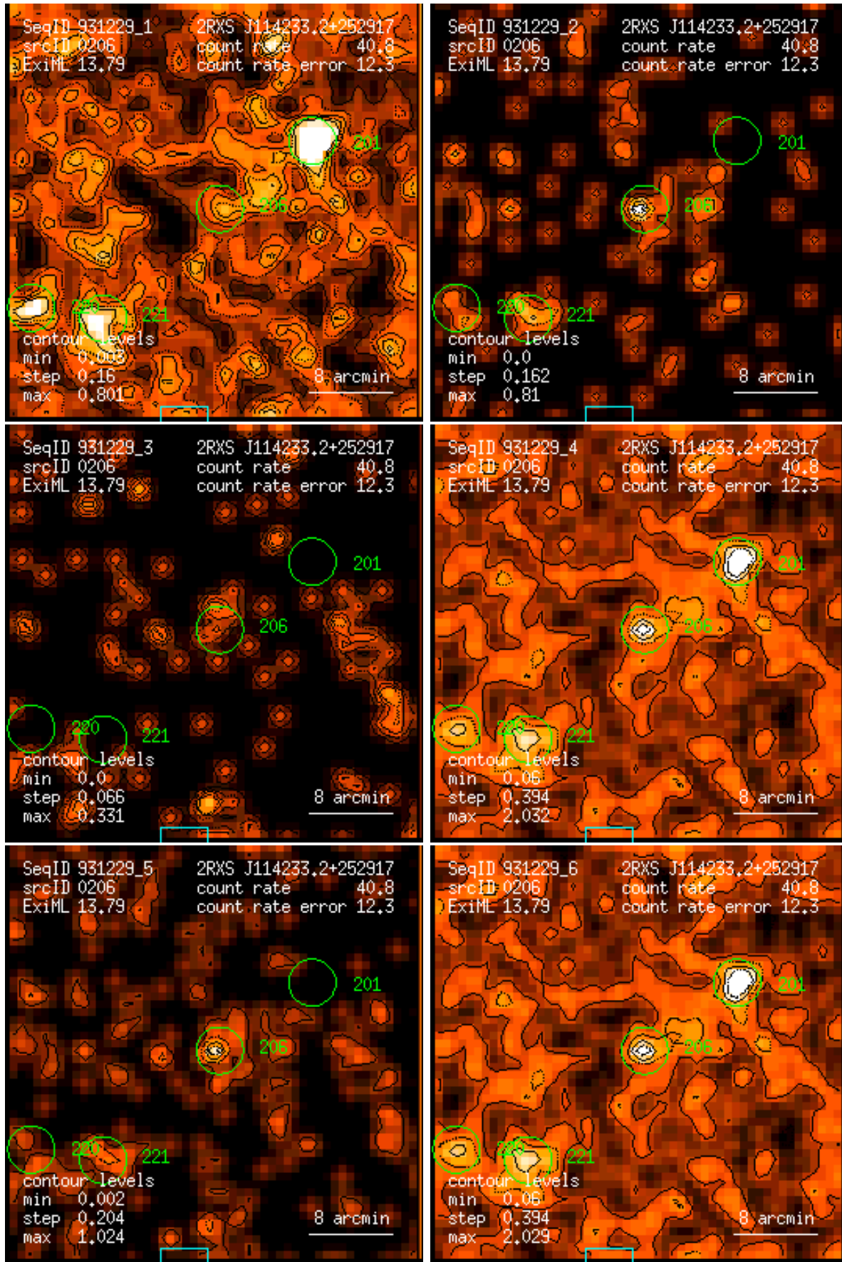
Figure 206: RASS 931229: detection 0206: band rate images, Gaussian filter: (1) PSPC channels 11 – 41, (2) 52 – 90, (3) 91 – 201, (4) 11 – 235, (5) 52 – 201, (6) 11 – 201. Broad band rates in counts/ks. Band rate contour levels in counts/ks/arcmin 2 .
