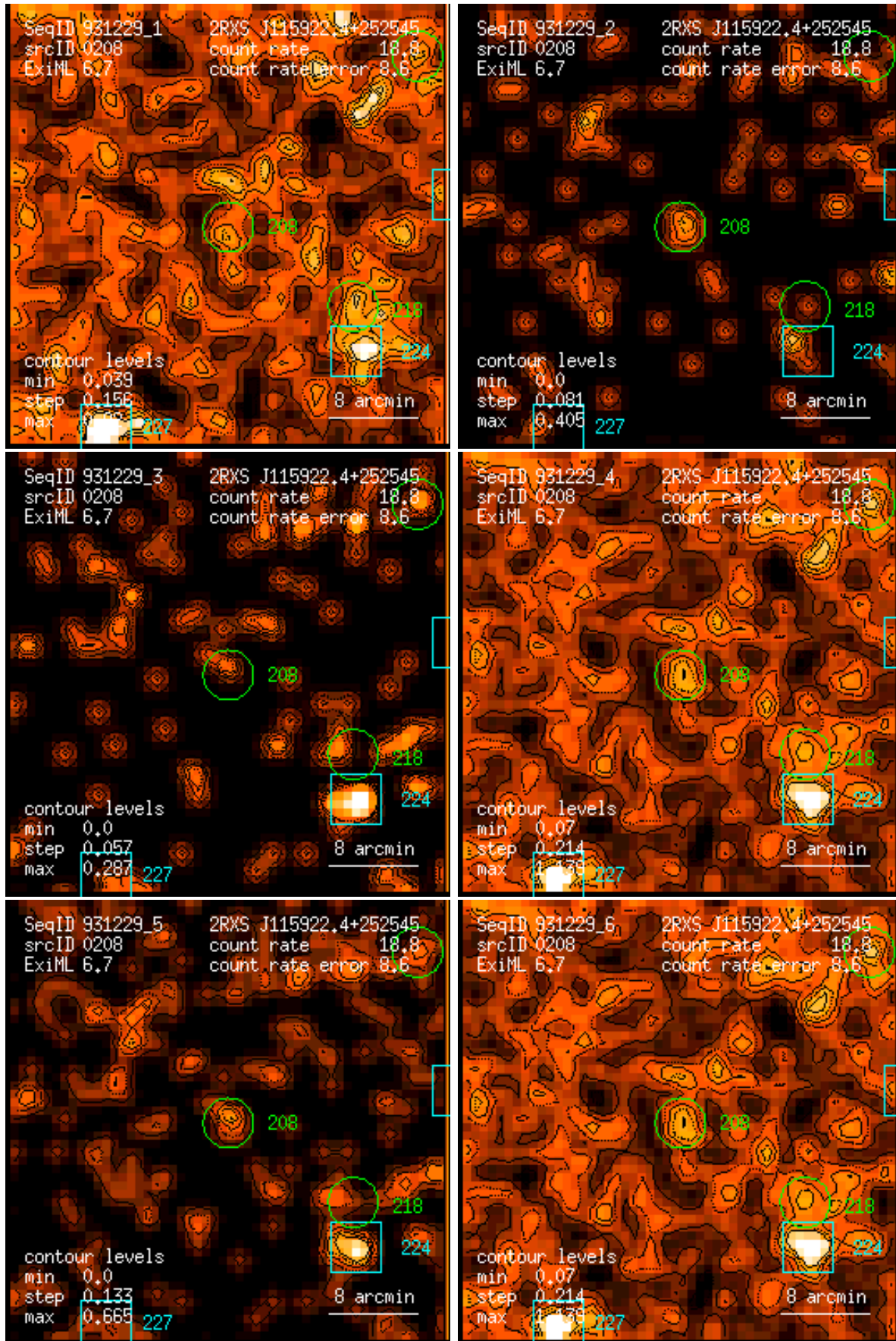
Figure 208: RASS 931229: detection 0208: band rate images, Gaussian filter: (1) PSPC channels 11 – 41, (2) 52 – 90, (3) 91 – 201, (4) 11 – 235, (5) 52 – 201, (6) 11 – 201. Broad band rates in counts/ks. Band rate contour levels in counts/ks/arcmin 2 .
