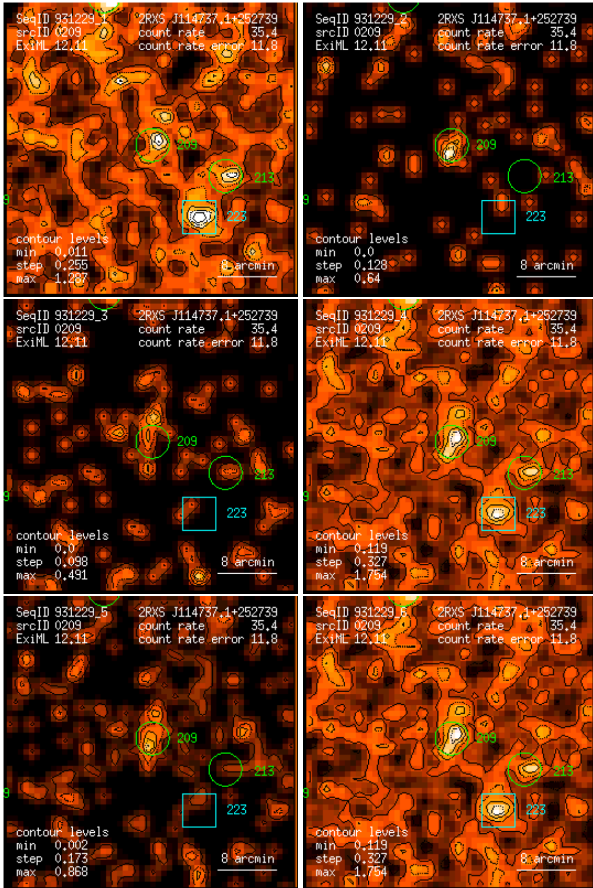
Figure 209: RASS 931229: detection 0209: band rate images, Gaussian filter: (1) PSPC channels 11 – 41, (2) 52 – 90, (3) 91 – 201, (4) 11 – 235, (5) 52 – 201, (6) 11 – 201. Broad band rates in counts/ks. Band rate contour levels in counts/ks/arcmin 2 .
