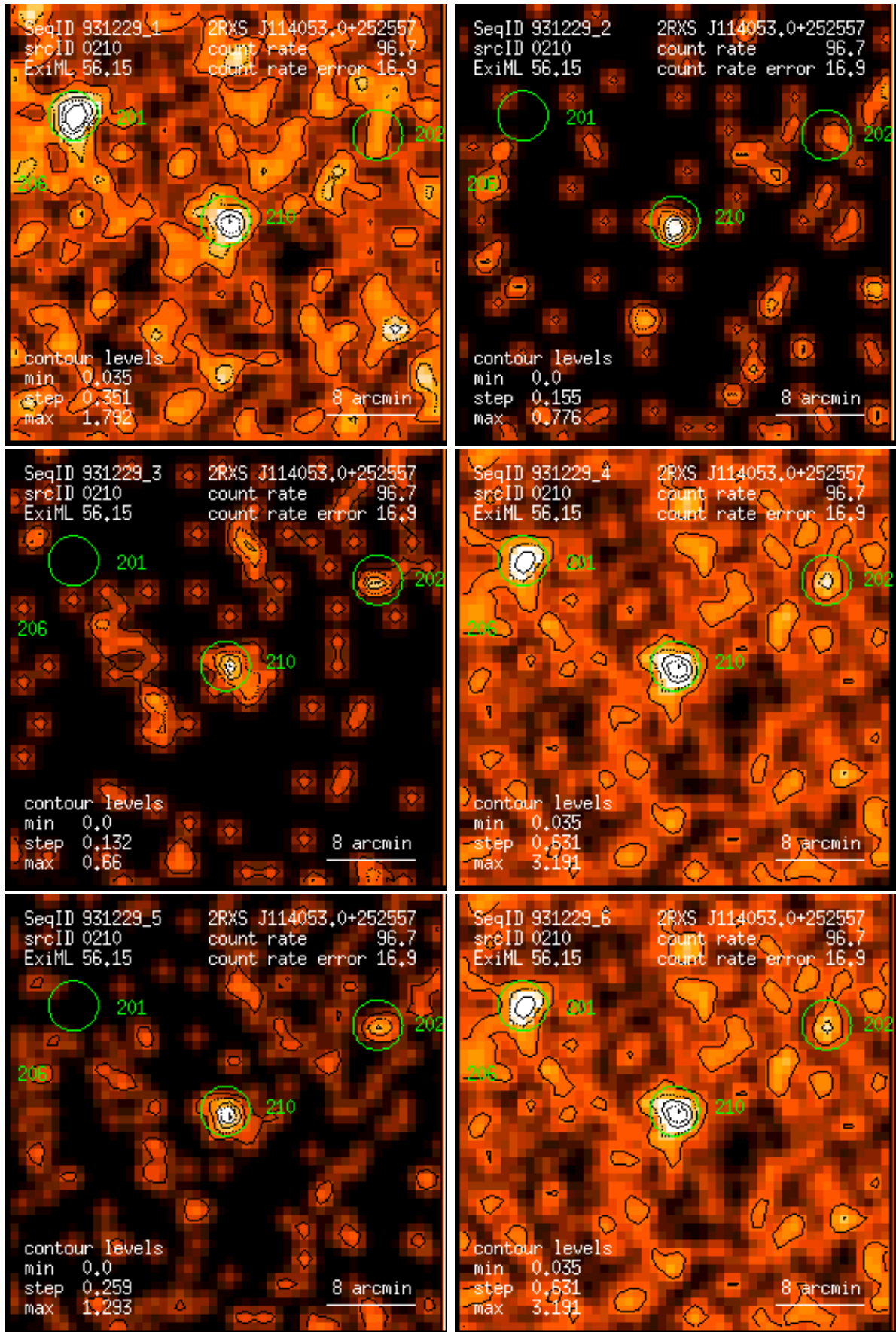
Figure 210: RASS 931229: detection 0210: band rate images, Gaussian filter: (1) PSPC channels 11 – 41, (2) 52 – 90, (3) 91 – 201, (4) 11 – 235, (5) 52 – 201, (6) 11 – 201. Broad band rates in counts/ks. Band rate contour levels in counts/ks/arcmin 2 .
