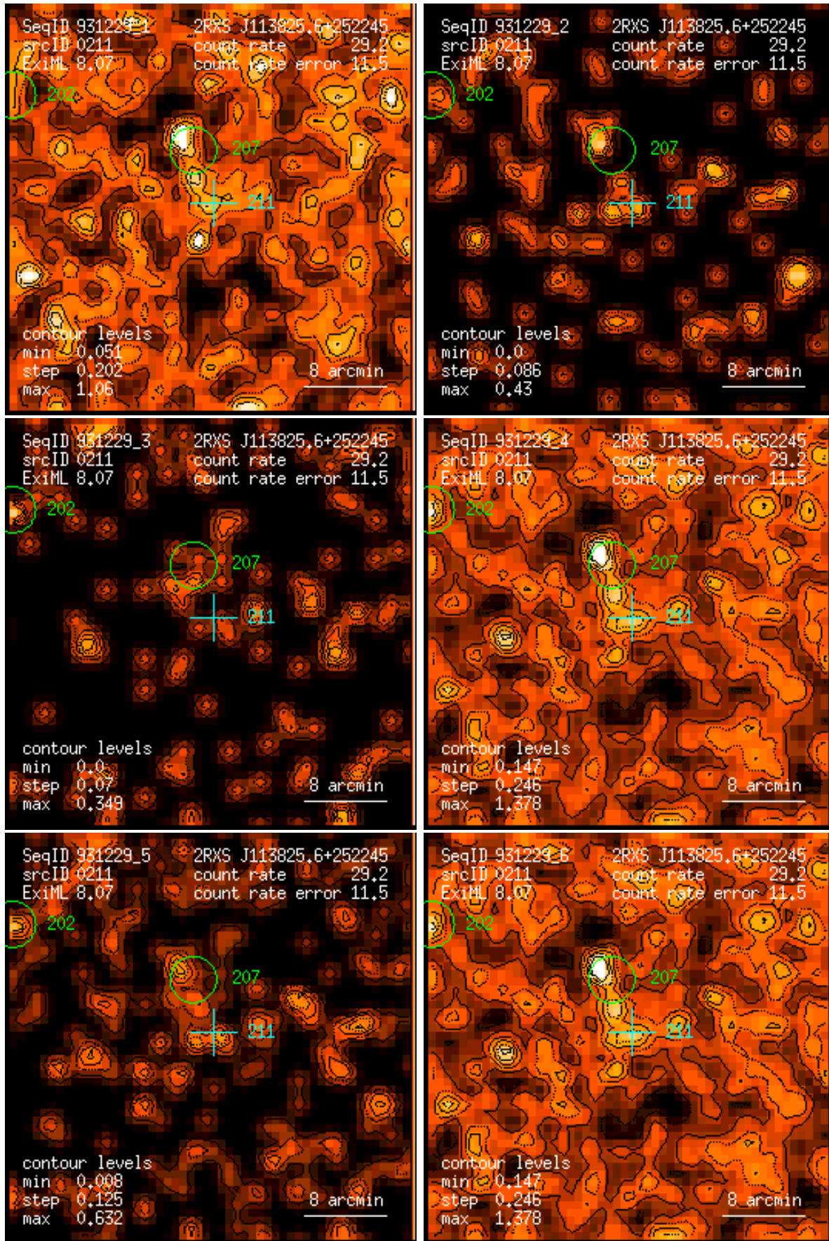
Figure 211: RASS 931229: detection 0211: band rate images, Gaussian filter: (1) PSPC channels 11 – 41, (2) 52 – 90, (3) 91 – 201, (4) 11 – 235, (5) 52 – 201, (6) 11 – 201. Broad band rates in counts/ks. Band rate contour levels in counts/ks/arcmin 2 .
