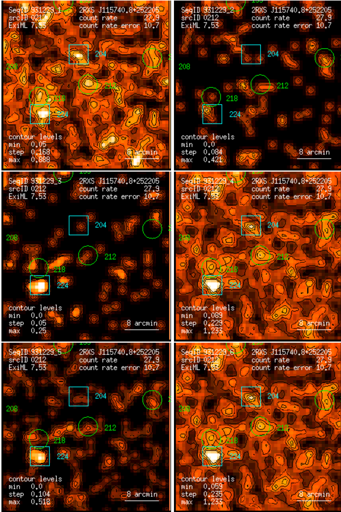
Figure 212: RASS 931229: detection 0212: band rate images, Gaussian filter: (1) PSPC channels 11 – 41, (2) 52 – 90, (3) 91 – 201, (4) 11 – 235, (5) 52 – 201, (6) 11 – 201. Broad band rates in counts/ks. Band rate contour levels in counts/ks/arcmin 2 .
