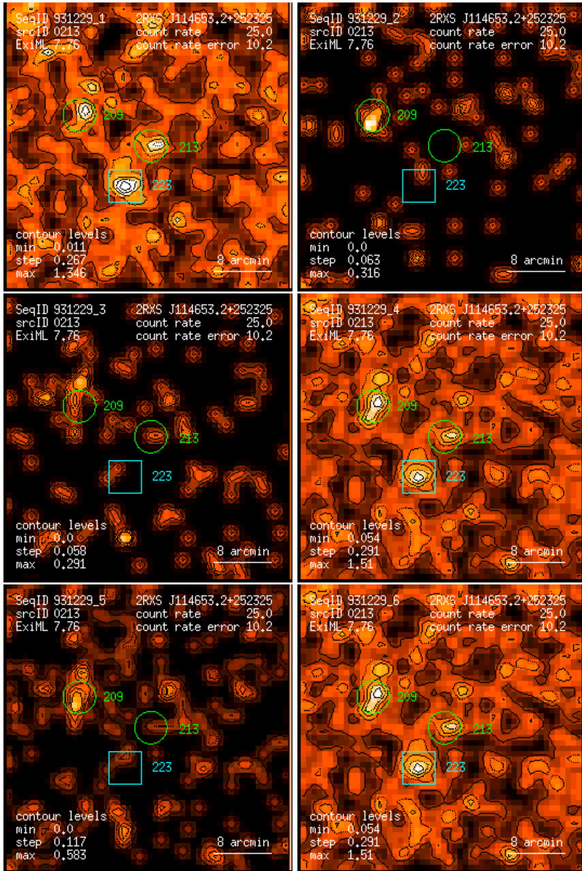
Figure 213: RASS 931229: detection 0213: band rate images, Gaussian filter: (1) PSPC channels 11 – 41, (2) 52 – 90, (3) 91 – 201, (4) 11 – 235, (5) 52 – 201, (6) 11 – 201. Broad band rates in counts/ks. Band rate contour levels in counts/ks/arcmin 2 .
