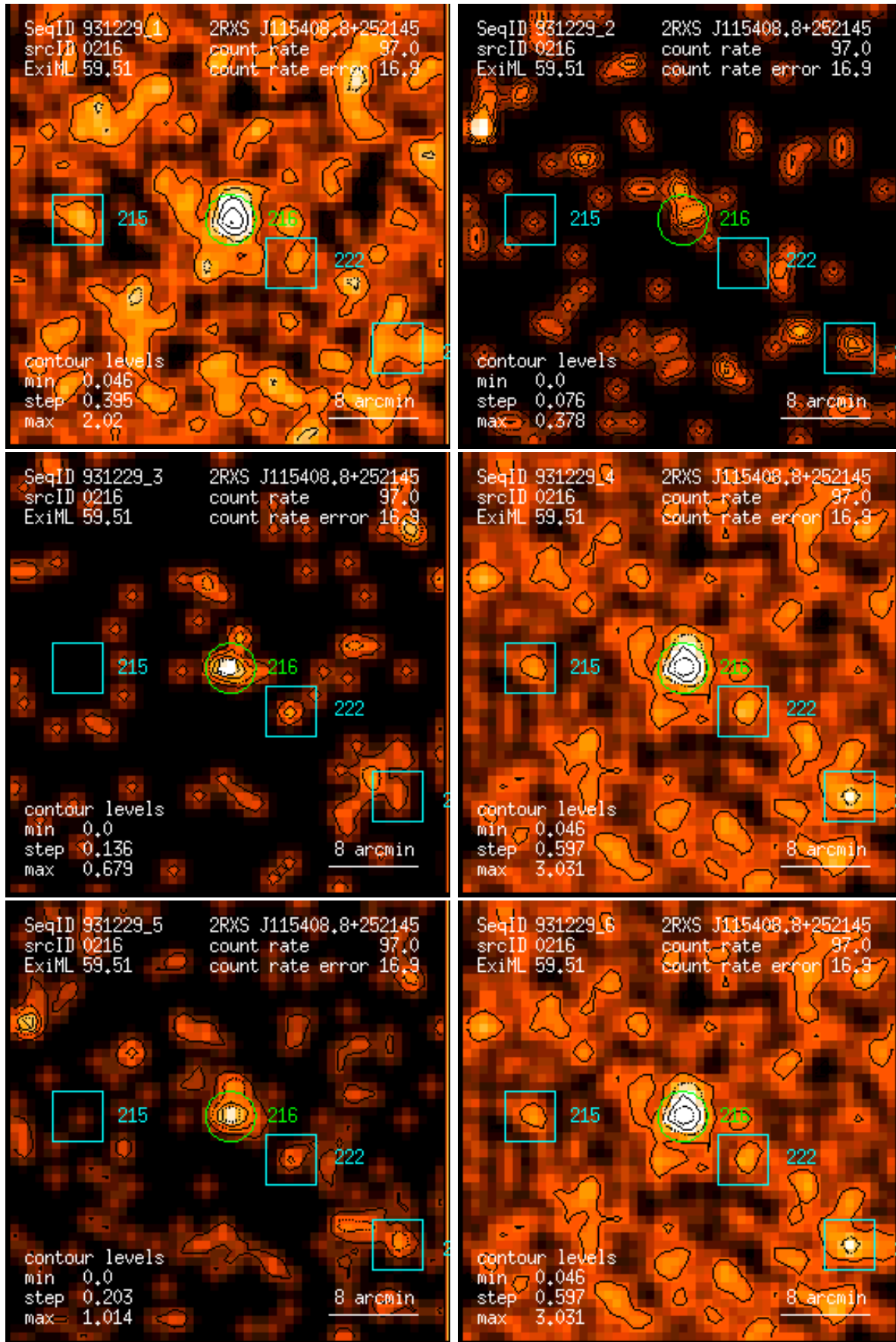
Figure 216: RASS 931229: detection 0216: band rate images, Gaussian filter: (1) PSPC channels 11 – 41, (2) 52 – 90, (3) 91 – 201, (4) 11 – 235, (5) 52 – 201, (6) 11 – 201. Broad band rates in counts/ks. Band rate contour levels in counts/ks/arcmin 2 .
