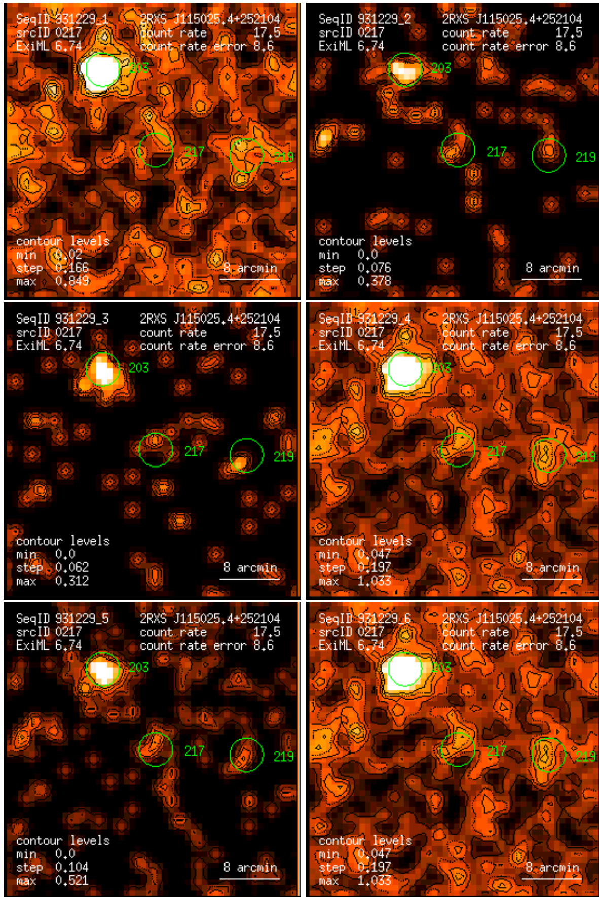
Figure 217: RASS 931229: detection 0217: band rate images, Gaussian filter: (1) PSPC channels 11 – 41, (2) 52 – 90, (3) 91 – 201, (4) 11 – 235, (5) 52 – 201, (6) 11 – 201. Broad band rates in counts/ks. Band rate contour levels in counts/ks/arcmin 2 .
