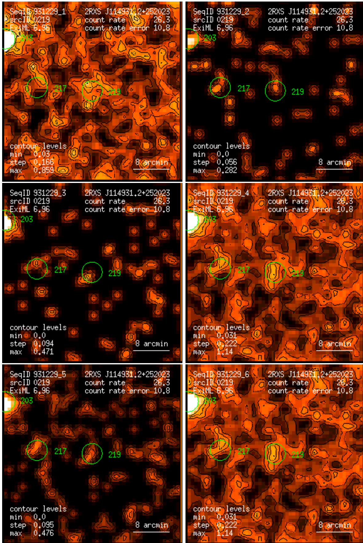
Figure 219: RASS 931229: detection 0219: band rate images, Gaussian filter: (1) PSPC channels 11 – 41, (2) 52 – 90, (3) 91 – 201, (4) 11 – 235, (5) 52 – 201, (6) 11 – 201. Broad band rates in counts/ks. Band rate contour levels in counts/ks/arcmin 2 .
