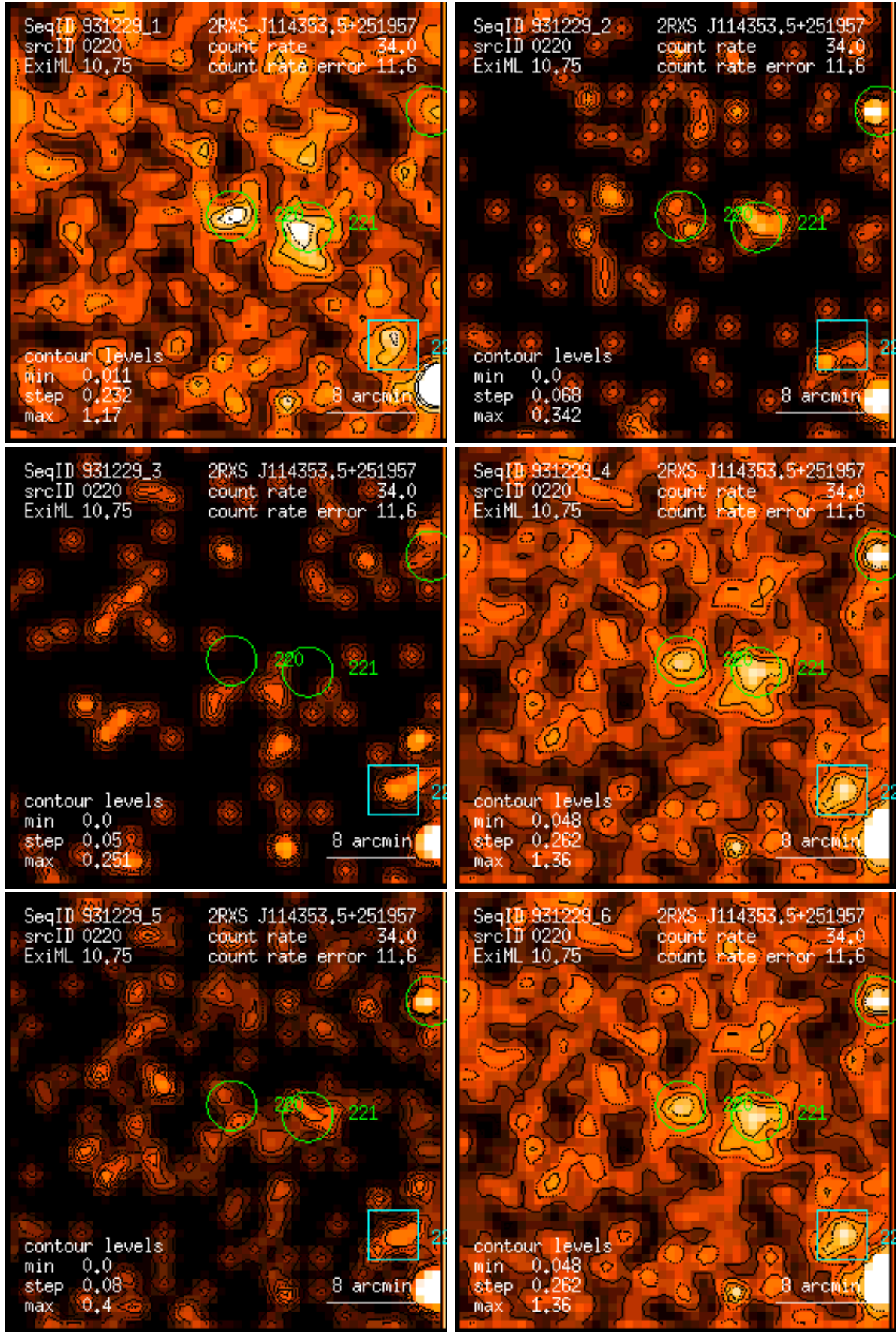
Figure 220: RASS 931229: detection 0220: band rate images, Gaussian filter: (1) PSPC channels 11 – 41, (2) 52 – 90, (3) 91 – 201, (4) 11 – 235, (5) 52 – 201, (6) 11 – 201. Broad band rates in counts/ks. Band rate contour levels in counts/ks/arcmin 2 .
