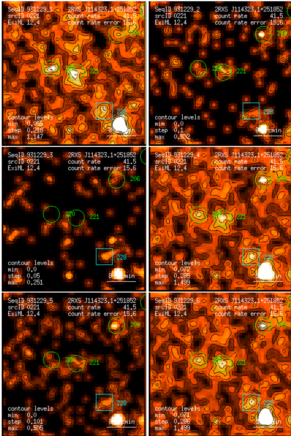
Figure 221: RASS 931229: detection 0221: band rate images, Gaussian filter: (1) PSPC channels 11 – 41, (2) 52 – 90, (3) 91 – 201, (4) 11 – 235, (5) 52 – 201, (6) 11 – 201. Broad band rates in counts/ks. Band rate contour levels in counts/ks/arcmin 2 .
