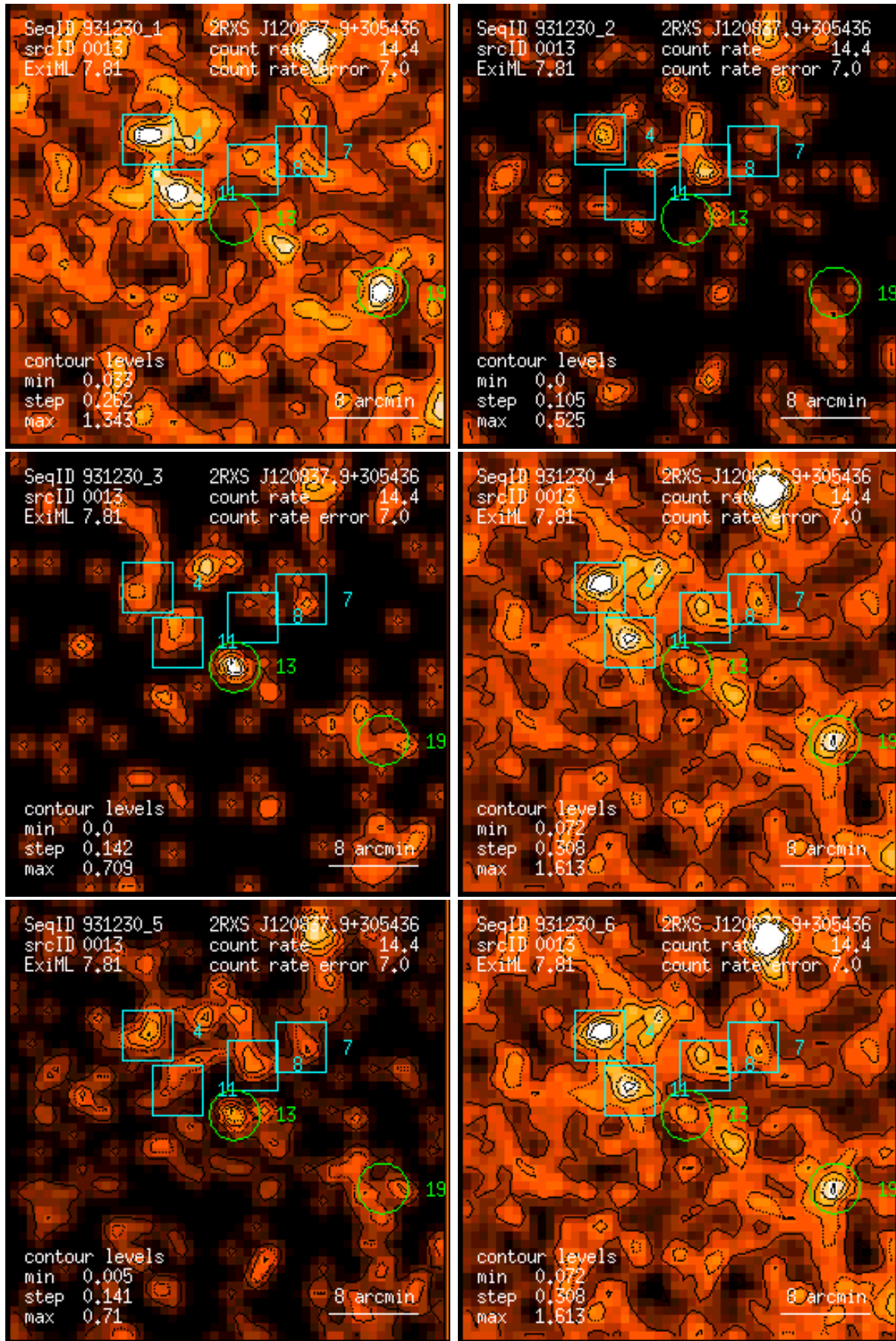
Figure 13: RASS 931230: detection 0013: band rate images, Gaussian filter: (1) PSPC channels 11 – 41, (2) 52 – 90, (3) 91 – 201, (4) 11 – 235, (5) 52 – 201, (6) 11 – 201. Broad band rates in counts/ks. Band rate contour levels in counts/ks/arcmin 2 .
