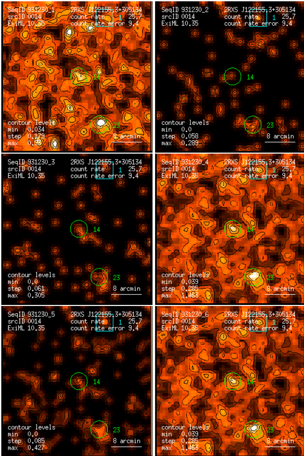
Figure 14: RASS 931230: detection 0014: band rate images, Gaussian filter: (1) PSPC channels 11 – 41, (2) 52 – 90, (3) 91 – 201, (4) 11 – 235, (5) 52 – 201, (6) 11 – 201. Broad band rates in counts/ks. Band rate contour levels in counts/ks/arcmin 2 .
