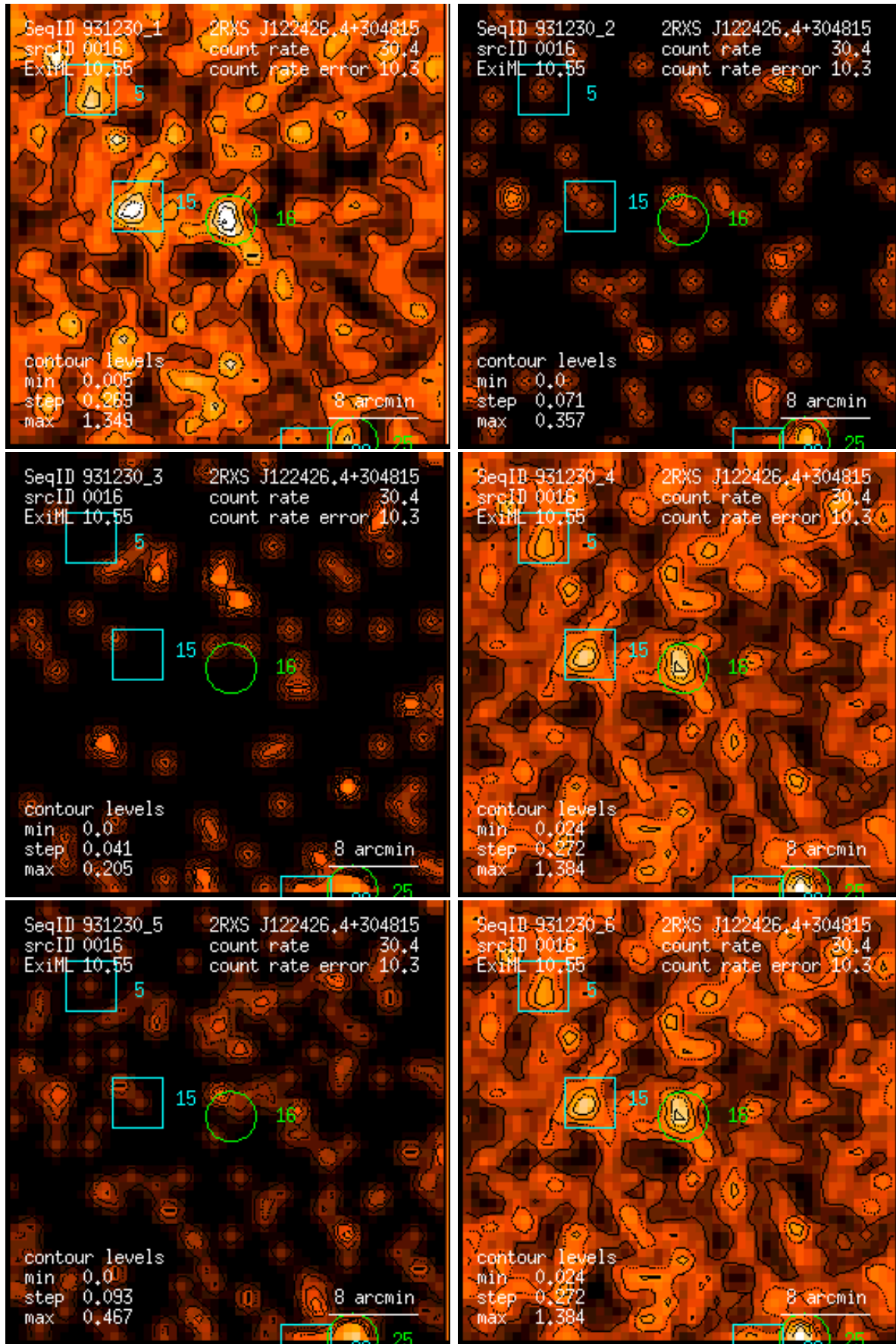
Figure 16: RASS 931230: detection 0016: band rate images, Gaussian filter: (1) PSPC channels 11 – 41, (2) 52 – 90, (3) 91 – 201, (4) 11 – 235, (5) 52 – 201, (6) 11 – 201. Broad band rates in counts/ks. Band rate contour levels in counts/ks/arcmin 2 .
