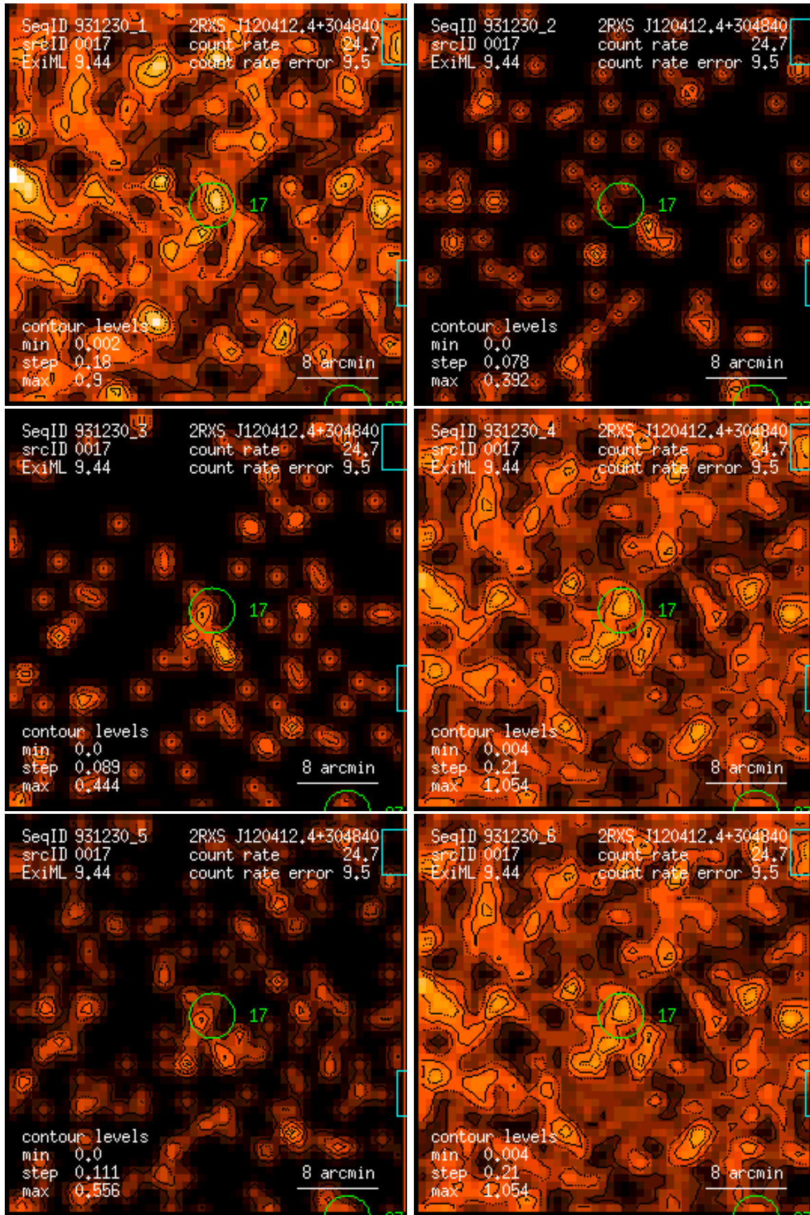
Figure 17: RASS 931230: detection 0017: band rate images, Gaussian filter: (1) PSPC channels 11 – 41, (2) 52 – 90, (3) 91 – 201, (4) 11 – 235, (5) 52 – 201, (6) 11 – 201. Broad band rates in counts/ks. Band rate contour levels in counts/ks/arcmin 2 .
