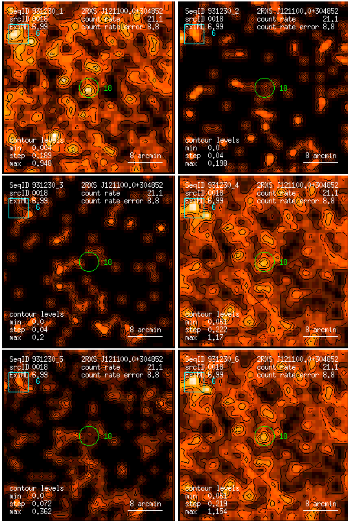
Figure 18: RASS 931230: detection 0018: band rate images, Gaussian filter: (1) PSPC channels 11 – 41, (2) 52 – 90, (3) 91 – 201, (4) 11 – 235, (5) 52 – 201, (6) 11 – 201. Broad band rates in counts/ks. Band rate contour levels in counts/ks/arcmin 2 .
