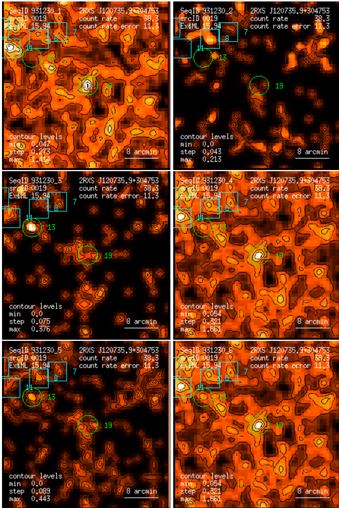
Figure 19: RASS 931230: detection 0019: band rate images, Gaussian filter: (1) PSPC channels 11 – 41, (2) 52 – 90, (3) 91 – 201, (4) 11 – 235, (5) 52 – 201, (6) 11 – 201. Broad band rates in counts/ks. Band rate contour levels in counts/ks/arcmin 2 .
