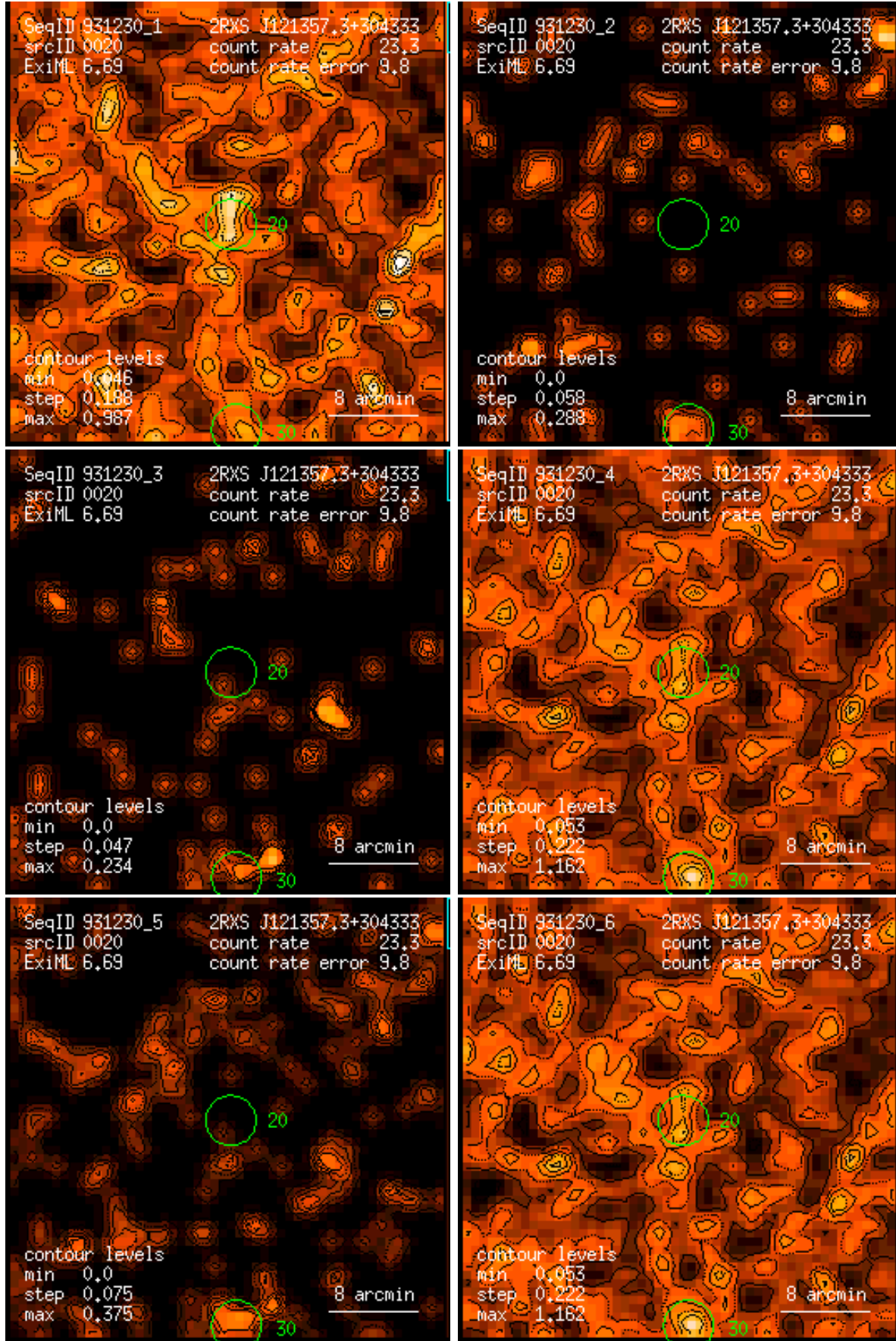
Figure 20: RASS 931230: detection 0020: band rate images, Gaussian filter: (1) PSPC channels 11 – 41, (2) 52 – 90, (3) 91 – 201, (4) 11 – 235, (5) 52 – 201, (6) 11 – 201. Broad band rates in counts/ks. Band rate contour levels in counts/ks/arcmin 2 .
