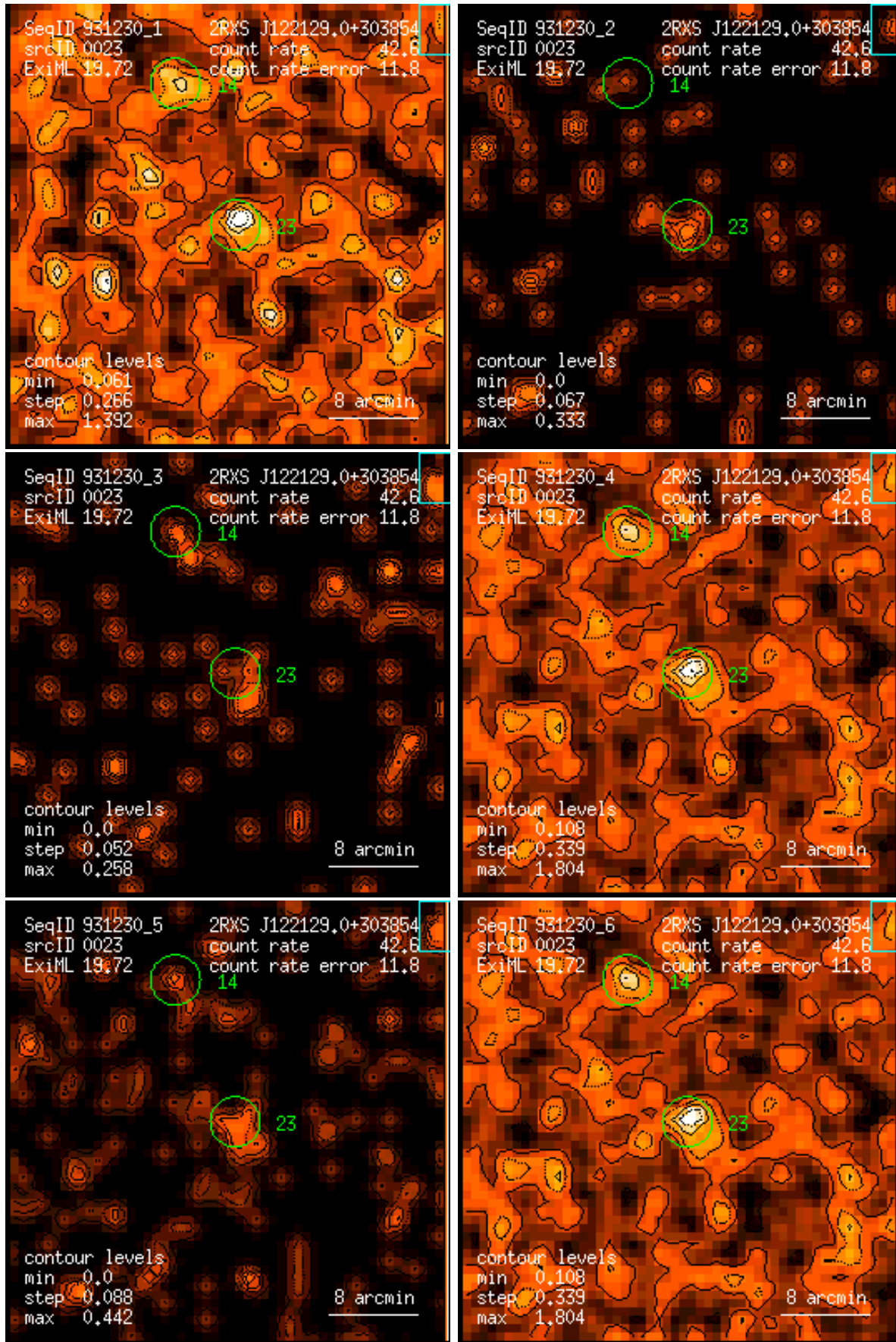
Figure 23: RASS 931230: detection 0023: band rate images, Gaussian filter: (1) PSPC channels 11 – 41, (2) 52 – 90, (3) 91 – 201, (4) 11 – 235, (5) 52 – 201, (6) 11 – 201. Broad band rates in counts/ks. Band rate contour levels in counts/ks/arcmin 2 .
