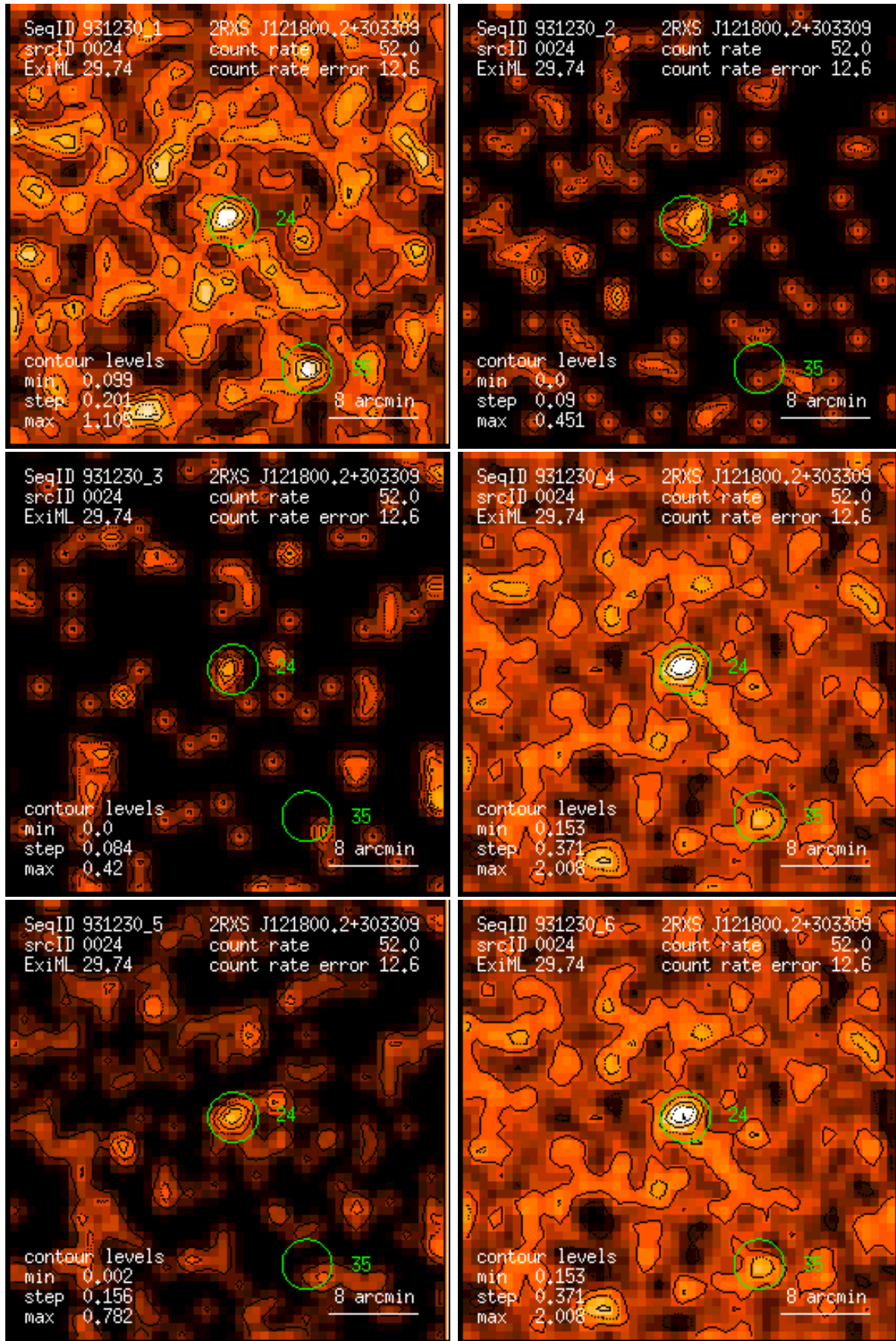
Figure 24: RASS 931230: detection 0024: band rate images, Gaussian filter: (1) PSPC channels 11 – 41, (2) 52 – 90, (3) 91 – 201, (4) 11 – 235, (5) 52 – 201, (6) 11 – 201. Broad band rates in counts/ks. Band rate contour levels in counts/ks/arcmin 2 .
