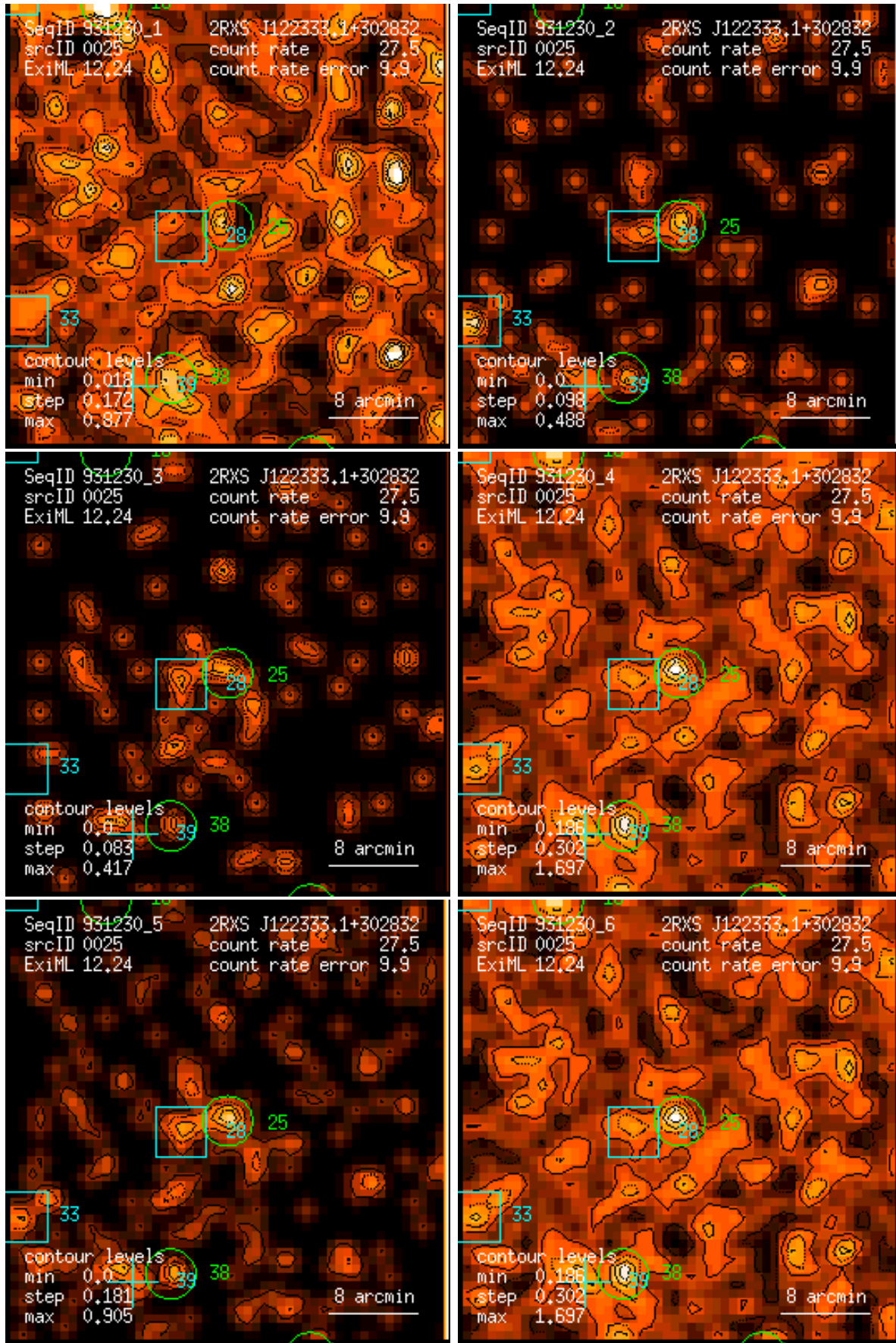
Figure 25: RASS 931230: detection 0025: band rate images, Gaussian filter: (1) PSPC channels 11 – 41, (2) 52 – 90, (3) 91 – 201, (4) 11 – 235, (5) 52 – 201, (6) 11 – 201. Broad band rates in counts/ks. Band rate contour levels in counts/ks/arcmin 2 .
