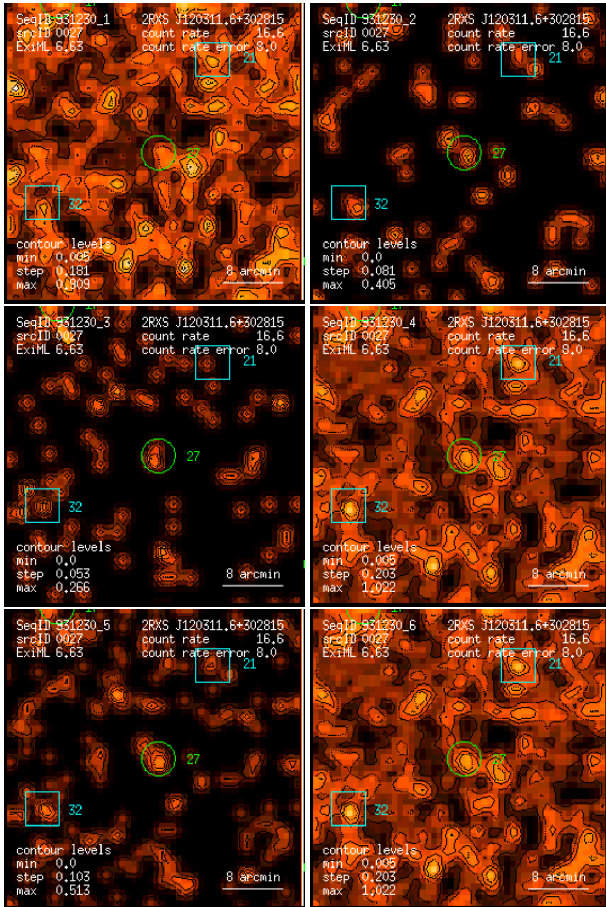
Figure 27: RASS 931230: detection 0027: band rate images, Gaussian filter: (1) PSPC channels 11 – 41, (2) 52 – 90, (3) 91 – 201, (4) 11 – 235, (5) 52 – 201, (6) 11 – 201. Broad band rates in counts/ks. Band rate contour levels in counts/ks/arcmin 2 .
