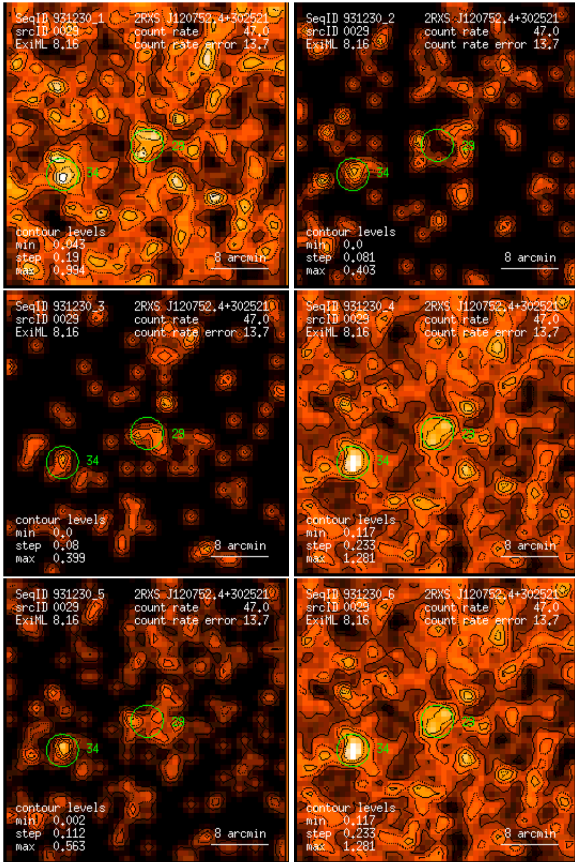
Figure 29: RASS 931230: detection 0029: band rate images, Gaussian filter: (1) PSPC channels 11 – 41, (2) 52 – 90, (3) 91 – 201, (4) 11 – 235, (5) 52 – 201, (6) 11 – 201. Broad band rates in counts/ks. Band rate contour levels in counts/ks/arcmin 2 .
