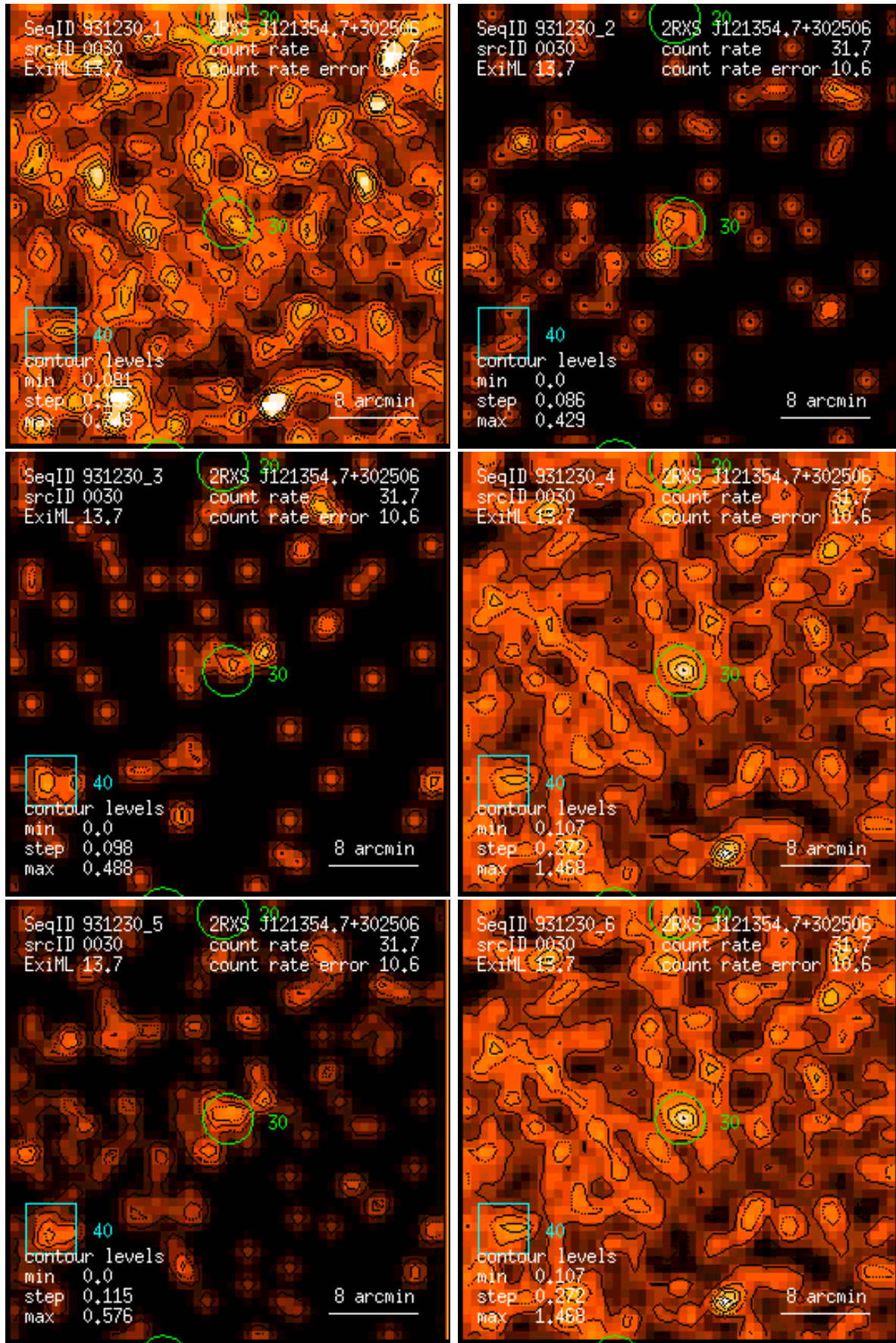
Figure 30: RASS 931230: detection 0030: band rate images, Gaussian filter: (1) PSPC channels 11 – 41, (2) 52 – 90, (3) 91 – 201, (4) 11 – 235, (5) 52 – 201, (6) 11 – 201. Broad band rates in counts/ks. Band rate contour levels in counts/ks/arcmin 2 .
