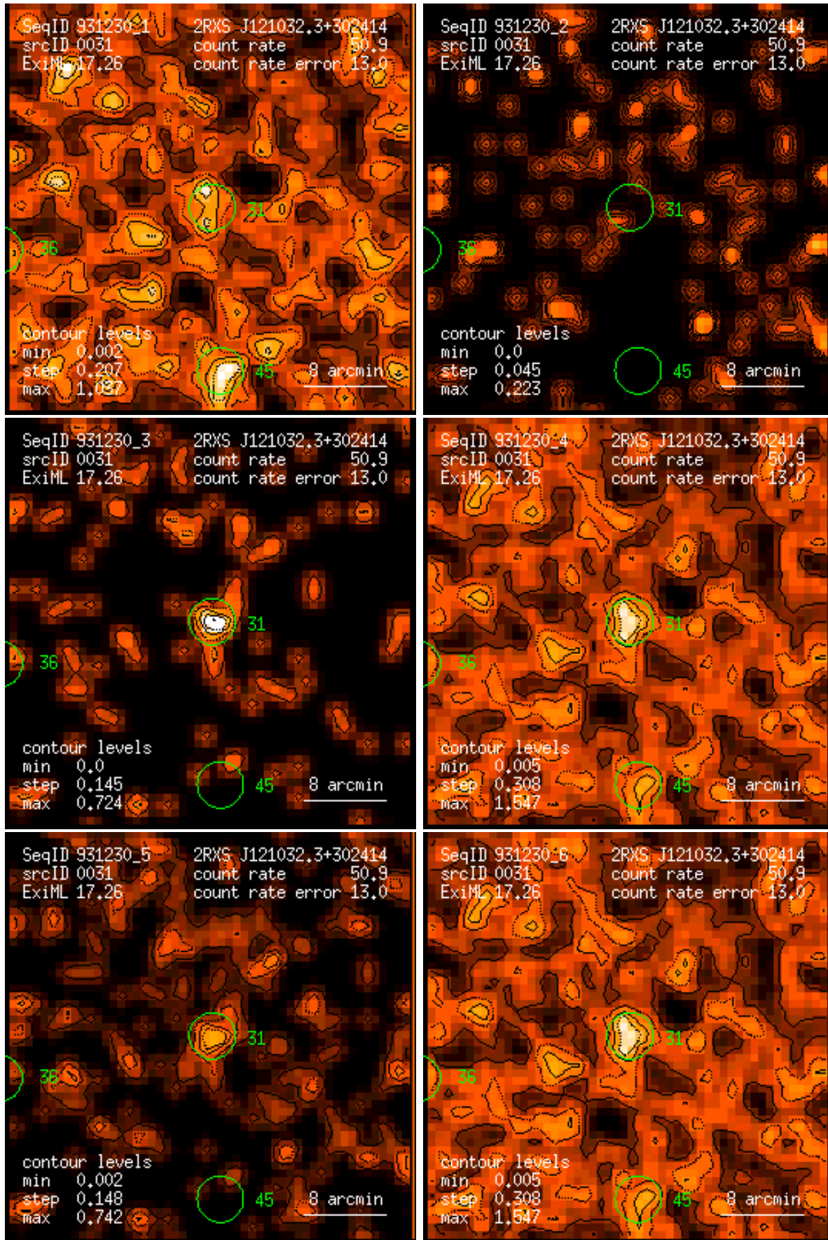
Figure 31: RASS 931230: detection 0031: band rate images, Gaussian filter: (1) PSPC channels 11 – 41, (2) 52 – 90, (3) 91 – 201, (4) 11 – 235, (5) 52 – 201, (6) 11 – 201. Broad band rates in counts/ks. Band rate contour levels in counts/ks/arcmin 2 .
