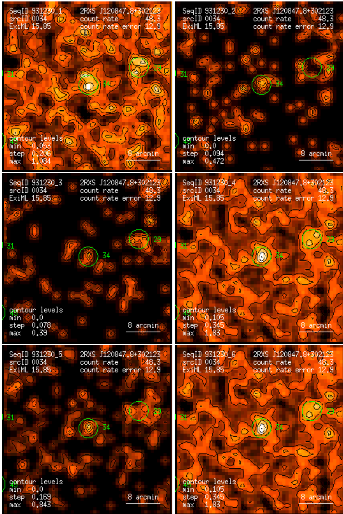
Figure 34: RASS 931230: detection 0034: band rate images, Gaussian filter: (1) PSPC channels 11 – 41, (2) 52 – 90, (3) 91 – 201, (4) 11 – 235, (5) 52 – 201, (6) 11 – 201. Broad band rates in counts/ks. Band rate contour levels in counts/ks/arcmin 2 .
