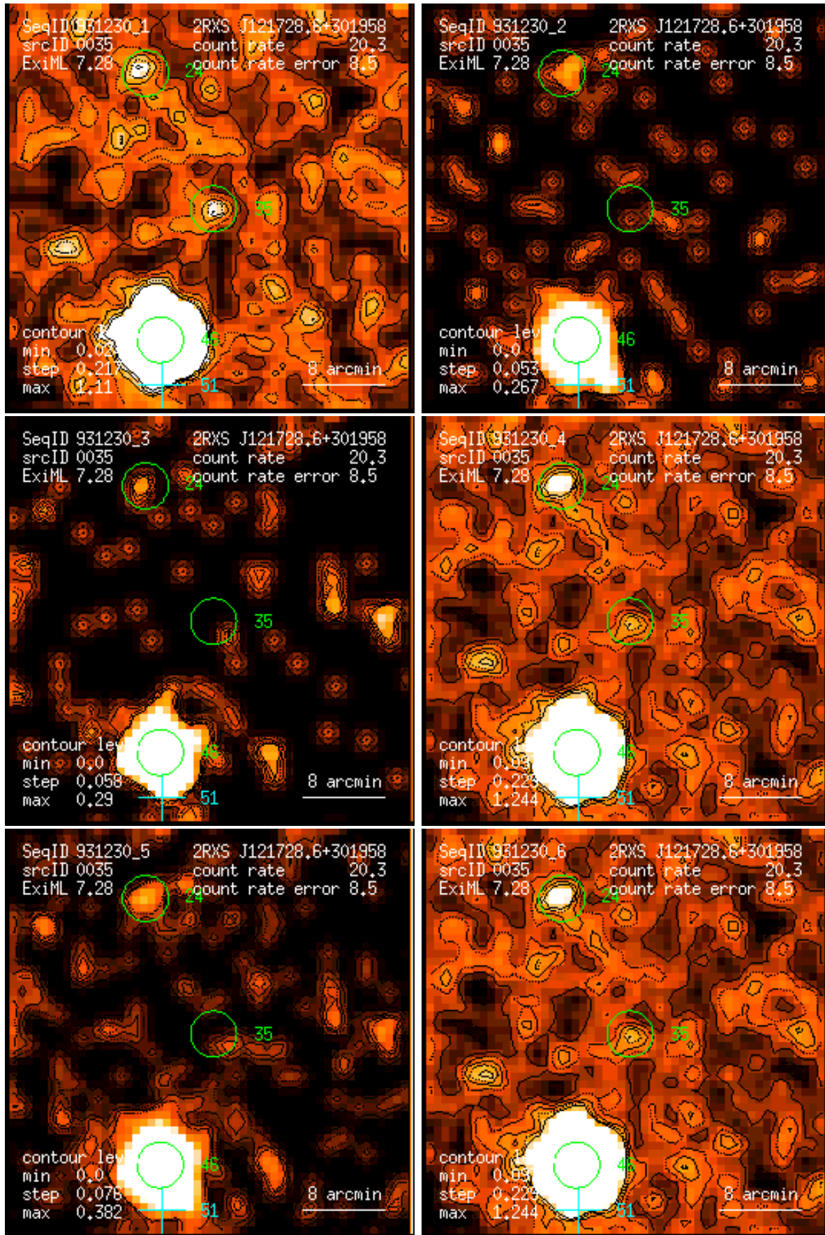
Figure 35: RASS 931230: detection 0035: band rate images, Gaussian filter: (1) PSPC channels 11 – 41, (2) 52 – 90, (3) 91 – 201, (4) 11 – 235, (5) 52 – 201, (6) 11 – 201. Broad band rates in counts/ks. Band rate contour levels in counts/ks/arcmin 2 .
