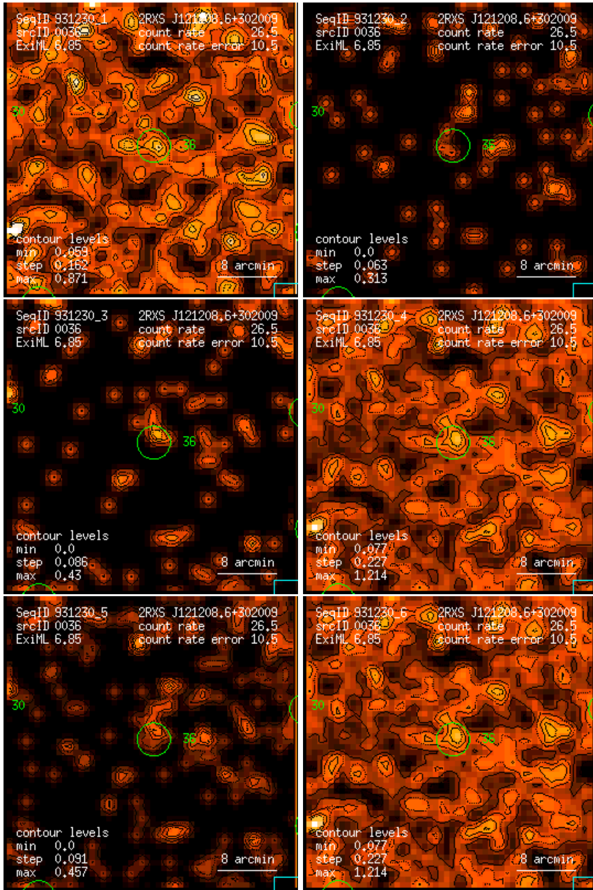
Figure 36: RASS 931230: detection 0036: band rate images, Gaussian filter: (1) PSPC channels 11 – 41, (2) 52 – 90, (3) 91 – 201, (4) 11 – 235, (5) 52 – 201, (6) 11 – 201. Broad band rates in counts/ks. Band rate contour levels in counts/ks/arcmin 2 .
