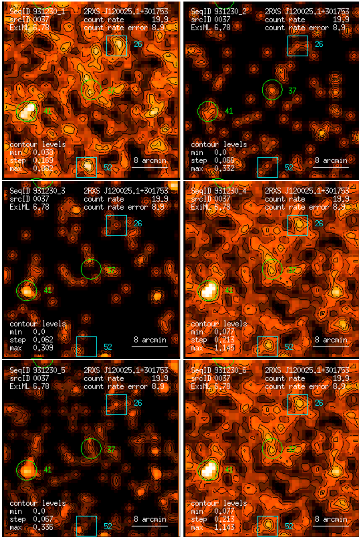
Figure 37: RASS 931230: detection 0037: band rate images, Gaussian filter: (1) PSPC channels 11 – 41, (2) 52 – 90, (3) 91 – 201, (4) 11 – 235, (5) 52 – 201, (6) 11 – 201. Broad band rates in counts/ks. Band rate contour levels in counts/ks/arcmin 2 .
