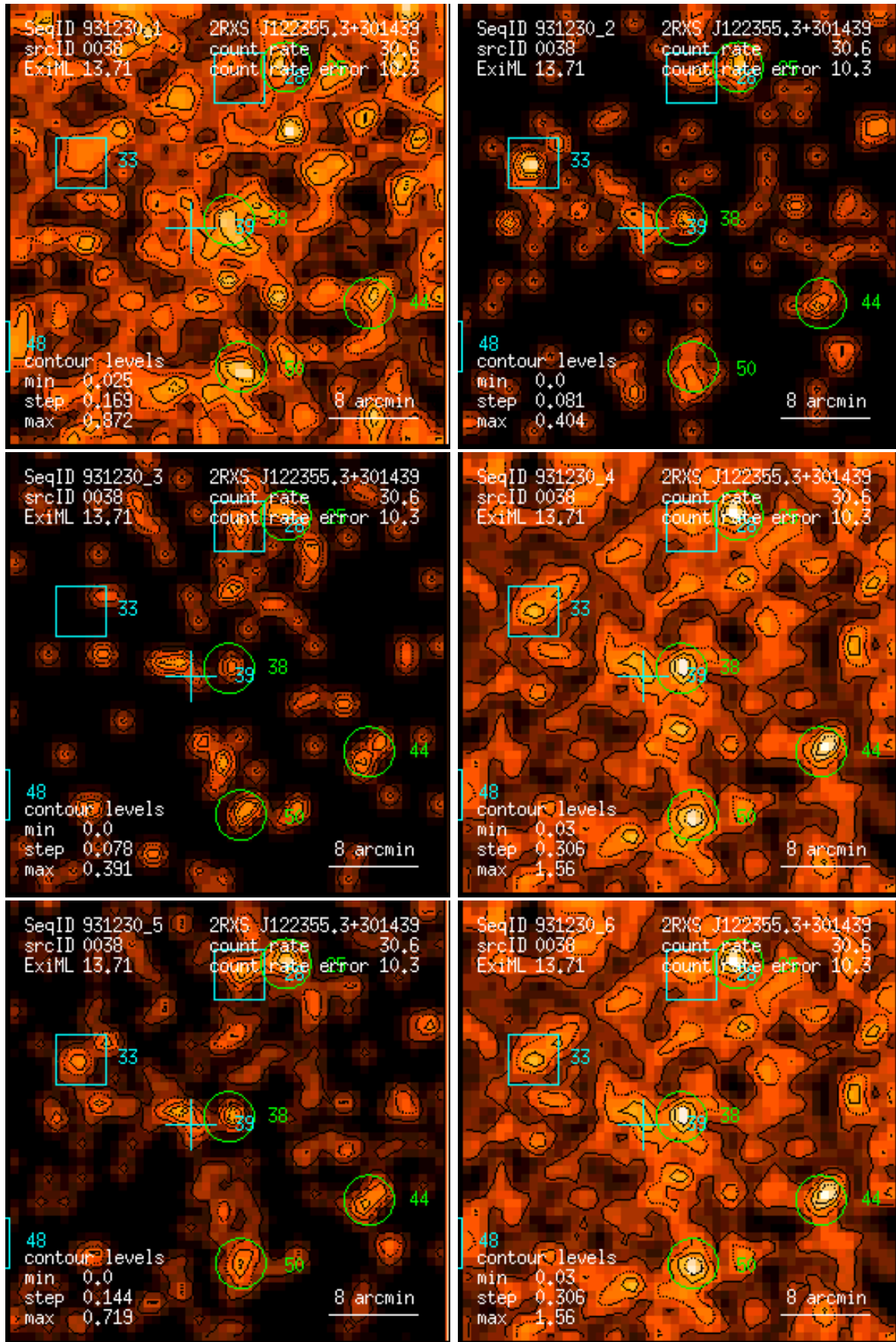
Figure 38: RASS 931230: detection 0038: band rate images, Gaussian filter: (1) PSPC channels 11 – 41, (2) 52 – 90, (3) 91 – 201, (4) 11 – 235, (5) 52 – 201, (6) 11 – 201. Broad band rates in counts/ks. Band rate contour levels in counts/ks/arcmin 2 .
