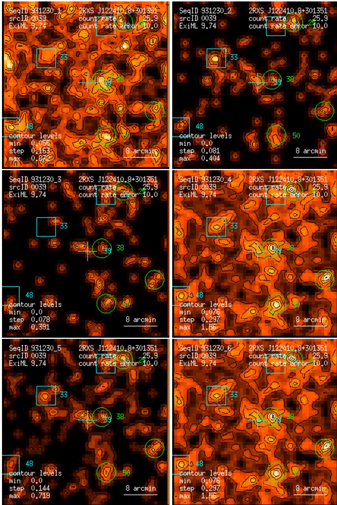
Figure 39: RASS 931230: detection 0039: band rate images, Gaussian filter: (1) PSPC channels 11 – 41, (2) 52 – 90, (3) 91 – 201, (4) 11 – 235, (5) 52 – 201, (6) 11 – 201. Broad band rates in counts/ks. Band rate contour levels in counts/ks/arcmin 2 .
