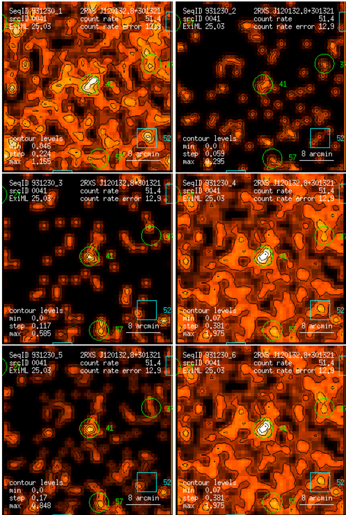
Figure 41: RASS 931230: detection 0041: band rate images, Gaussian filter: (1) PSPC channels 11 – 41, (2) 52 – 90, (3) 91 – 201, (4) 11 – 235, (5) 52 – 201, (6) 11 – 201. Broad band rates in counts/ks. Band rate contour levels in counts/ks/arcmin 2 .
