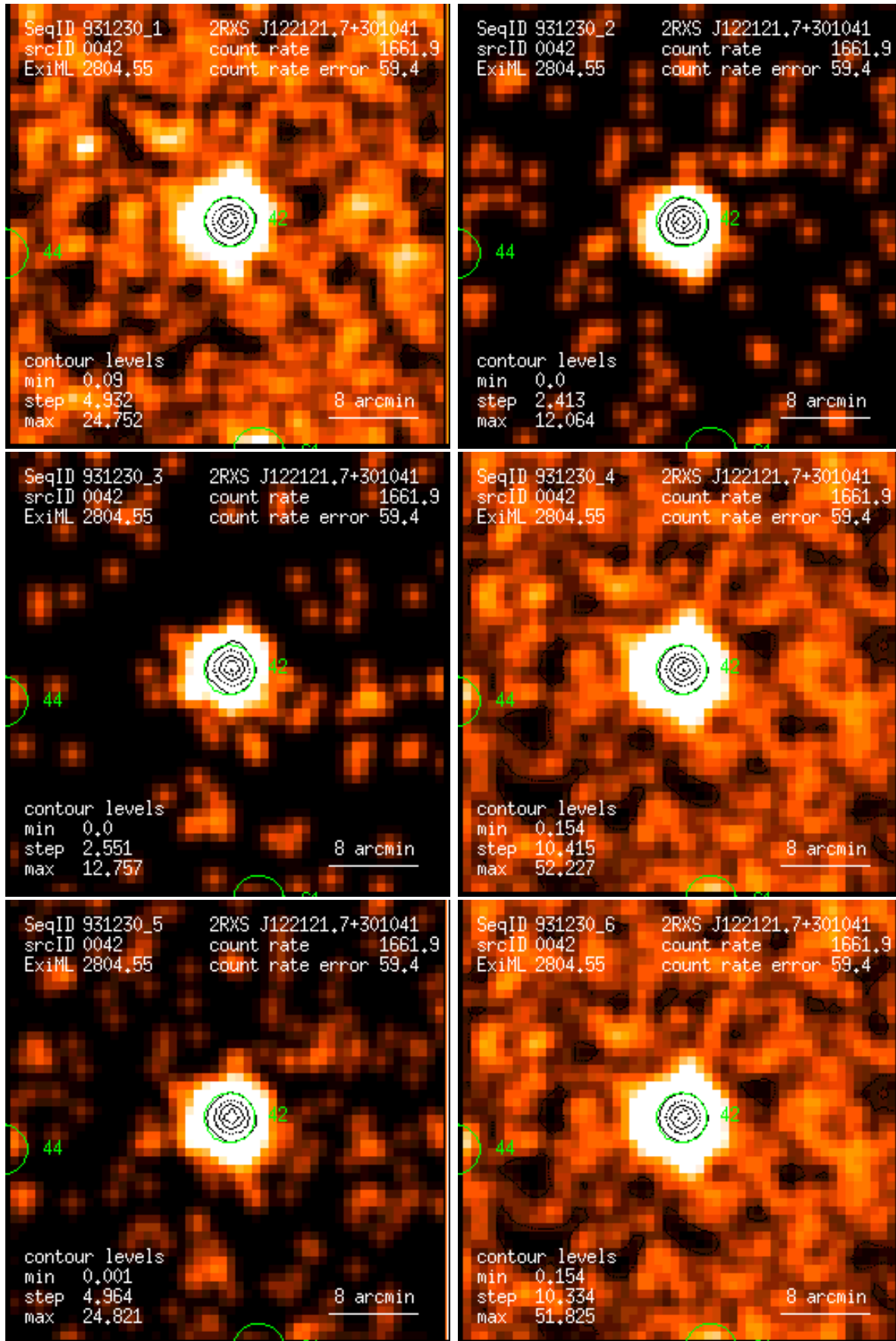
Figure 42: RASS 931230: detection 0042: band rate images, Gaussian filter: (1) PSPC channels 11 – 41, (2) 52 – 90, (3) 91 – 201, (4) 11 – 235, (5) 52 – 201, (6) 11 – 201. Broad band rates in counts/ks. Band rate contour levels in counts/ks/arcmin 2 .
