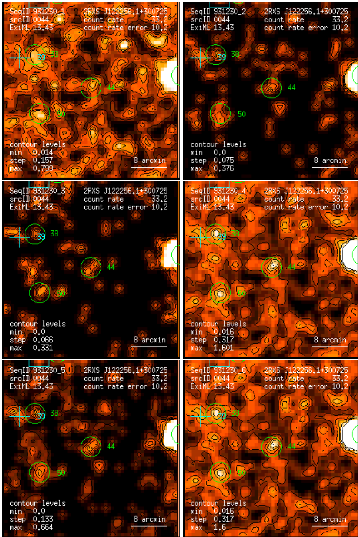
Figure 44: RASS 931230: detection 0044: band rate images, Gaussian filter: (1) PSPC channels 11 – 41, (2) 52 – 90, (3) 91 – 201, (4) 11 – 235, (5) 52 – 201, (6) 11 – 201. Broad band rates in counts/ks. Band rate contour levels in counts/ks/arcmin 2 .
