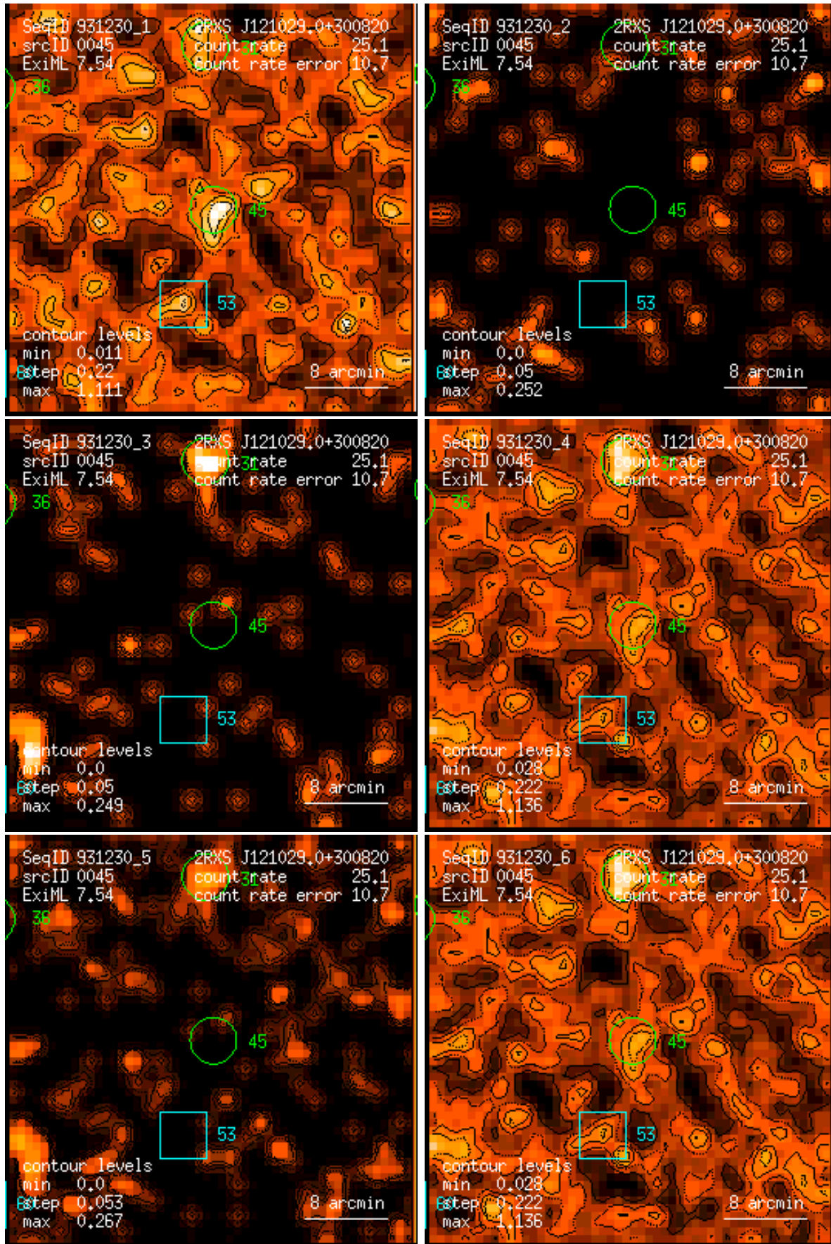
Figure 45: RASS 931230: detection 0045: band rate images, Gaussian filter: (1) PSPC channels 11 – 41, (2) 52 – 90, (3) 91 – 201, (4) 11 – 235, (5) 52 – 201, (6) 11 – 201. Broad band rates in counts/ks. Band rate contour levels in counts/ks/arcmin 2 .
