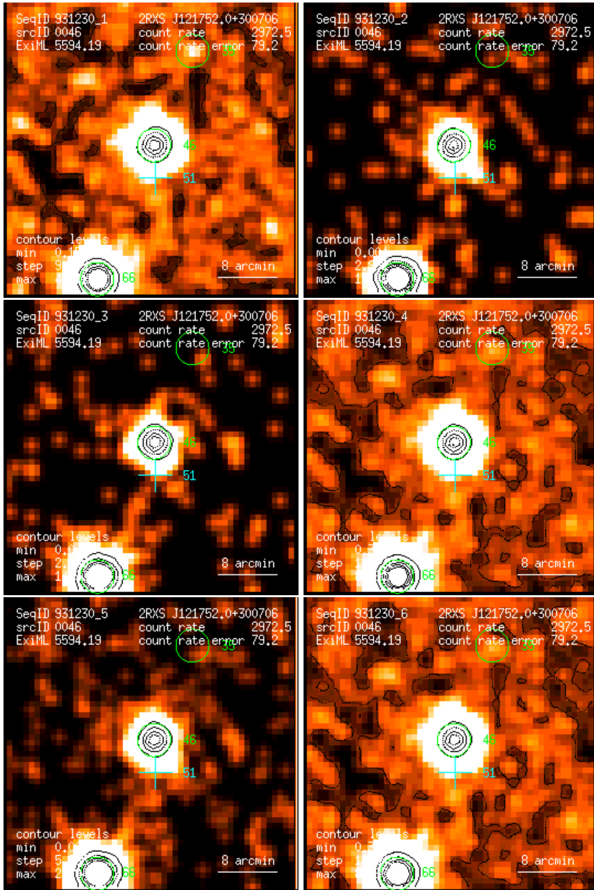
Figure 46: RASS 931230: detection 0046: band rate images, Gaussian filter: (1) PSPC channels 11 – 41, (2) 52 – 90, (3) 91 – 201, (4) 11 – 235, (5) 52 – 201, (6) 11 – 201. Broad band rates in counts/ks. Band rate contour levels in counts/ks/arcmin 2 .
