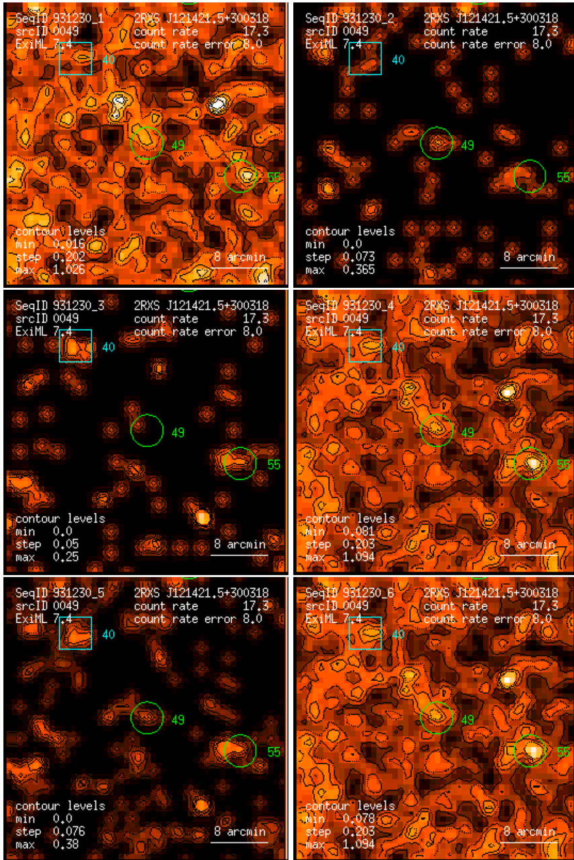
Figure 49: RASS 931230: detection 0049: band rate images, Gaussian filter: (1) PSPC channels 11 – 41, (2) 52 – 90, (3) 91 – 201, (4) 11 – 235, (5) 52 – 201, (6) 11 – 201. Broad band rates in counts/ks. Band rate contour levels in counts/ks/arcmin 2 .
