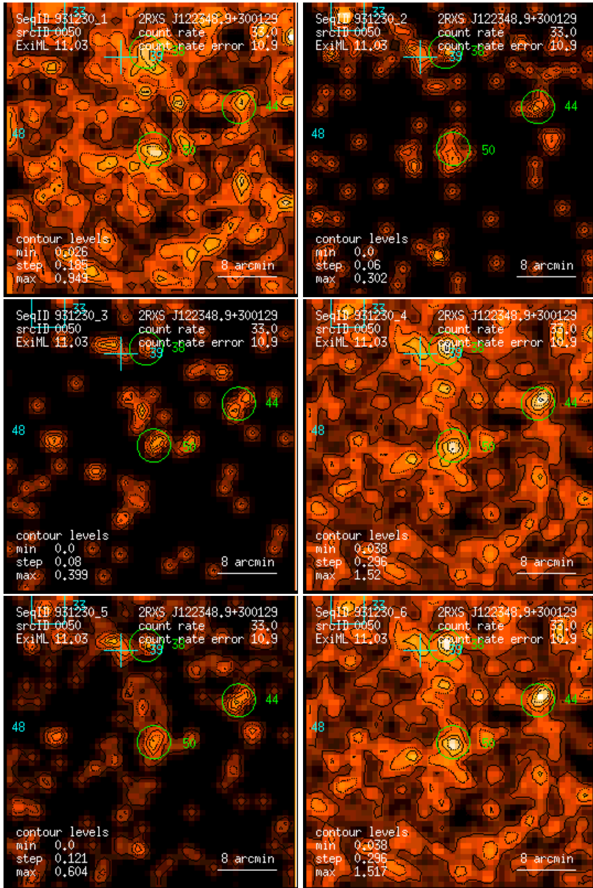
Figure 50: RASS 931230: detection 0050: band rate images, Gaussian filter: (1) PSPC channels 11 – 41, (2) 52 – 90, (3) 91 – 201, (4) 11 – 235, (5) 52 – 201, (6) 11 – 201. Broad band rates in counts/ks. Band rate contour levels in counts/ks/arcmin 2 .
