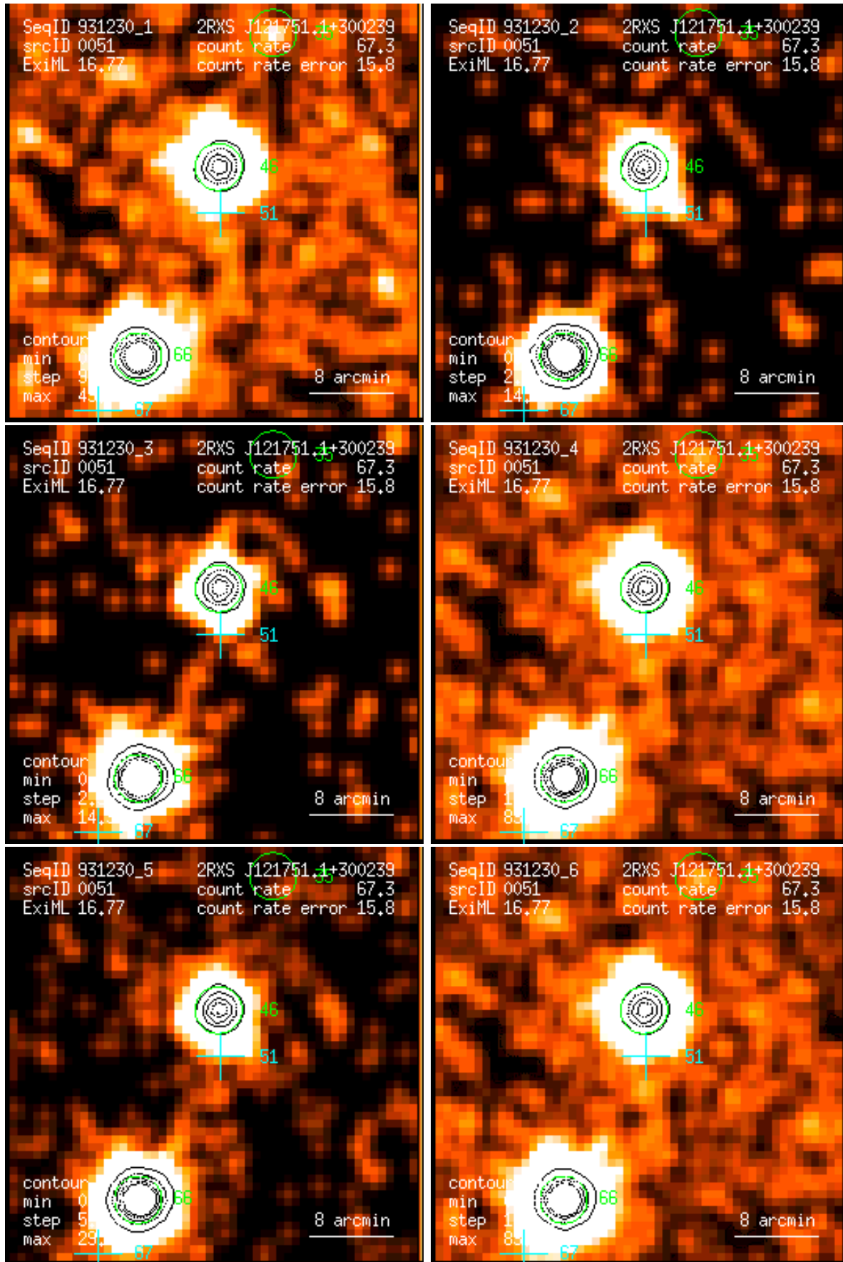
Figure 51: RASS 931230: detection 0051: band rate images, Gaussian filter: (1) PSPC channels 11 – 41, (2) 52 – 90, (3) 91 – 201, (4) 11 – 235, (5) 52 – 201, (6) 11 – 201. Broad band rates in counts/ks. Band rate contour levels in counts/ks/arcmin 2 .
