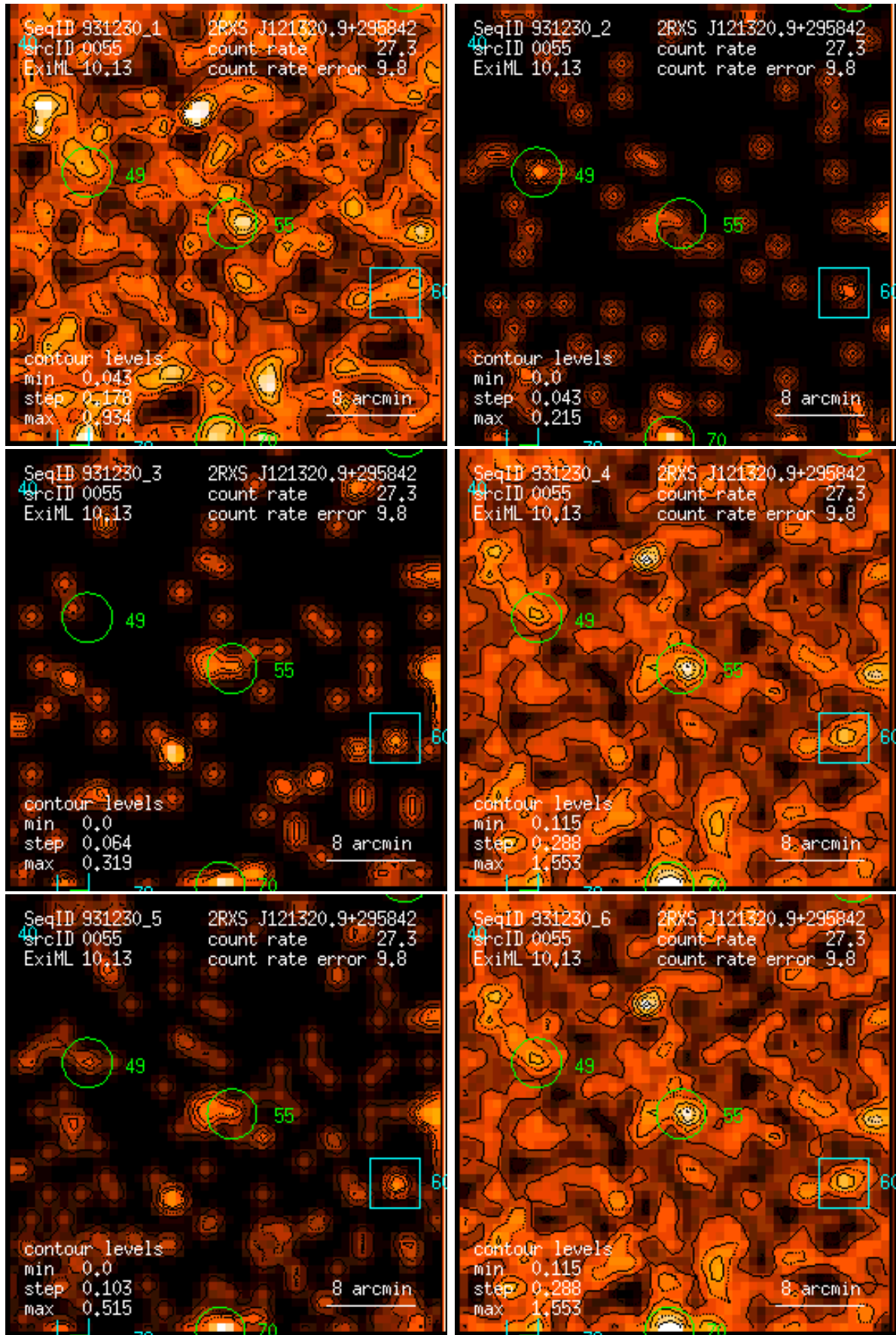
Figure 55: RASS 931230: detection 0055: band rate images, Gaussian filter: (1) PSPC channels 11 – 41, (2) 52 – 90, (3) 91 – 201, (4) 11 – 235, (5) 52 – 201, (6) 11 – 201. Broad band rates in counts/ks. Band rate contour levels in counts/ks/arcmin 2 .
