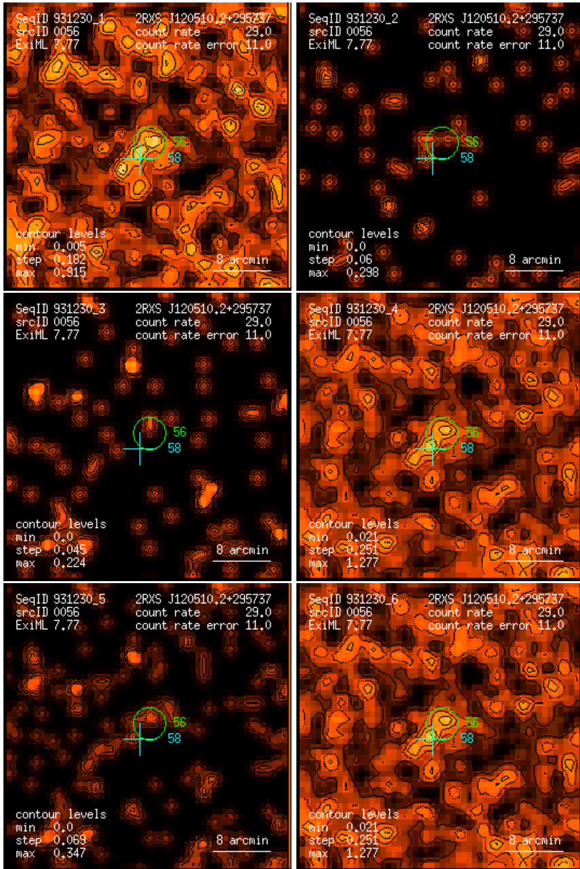
Figure 56: RASS 931230: detection 0056: band rate images, Gaussian filter: (1) PSPC channels 11 – 41, (2) 52 – 90, (3) 91 – 201, (4) 11 – 235, (5) 52 – 201, (6) 11 – 201. Broad band rates in counts/ks. Band rate contour levels in counts/ks/arcmin 2 .
