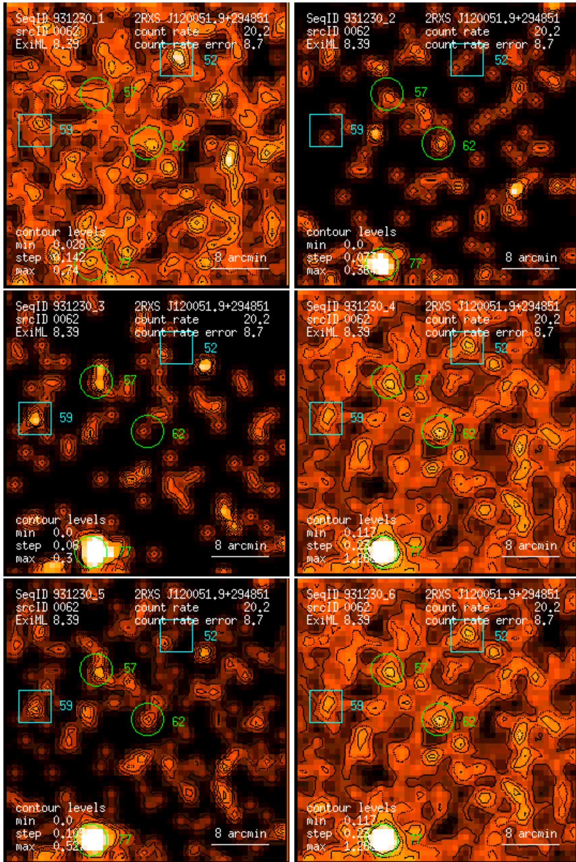
Figure 62: RASS 931230: detection 0062: band rate images, Gaussian filter: (1) PSPC channels 11 – 41, (2) 52 – 90, (3) 91 – 201, (4) 11 – 235, (5) 52 – 201, (6) 11 – 201. Broad band rates in counts/ks. Band rate contour levels in counts/ks/arcmin 2 .
